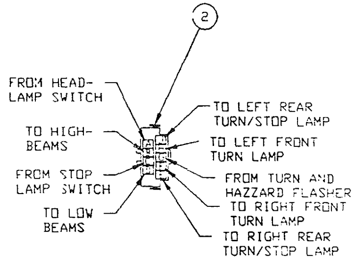
TURN/DIMMER SWITCH CONNECTOR VIEWED IN DIRECTION OF ARROW
