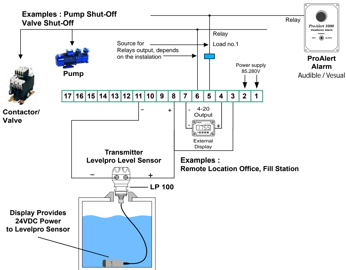
Wiring to the Levelpro Series Tank Level Controller
