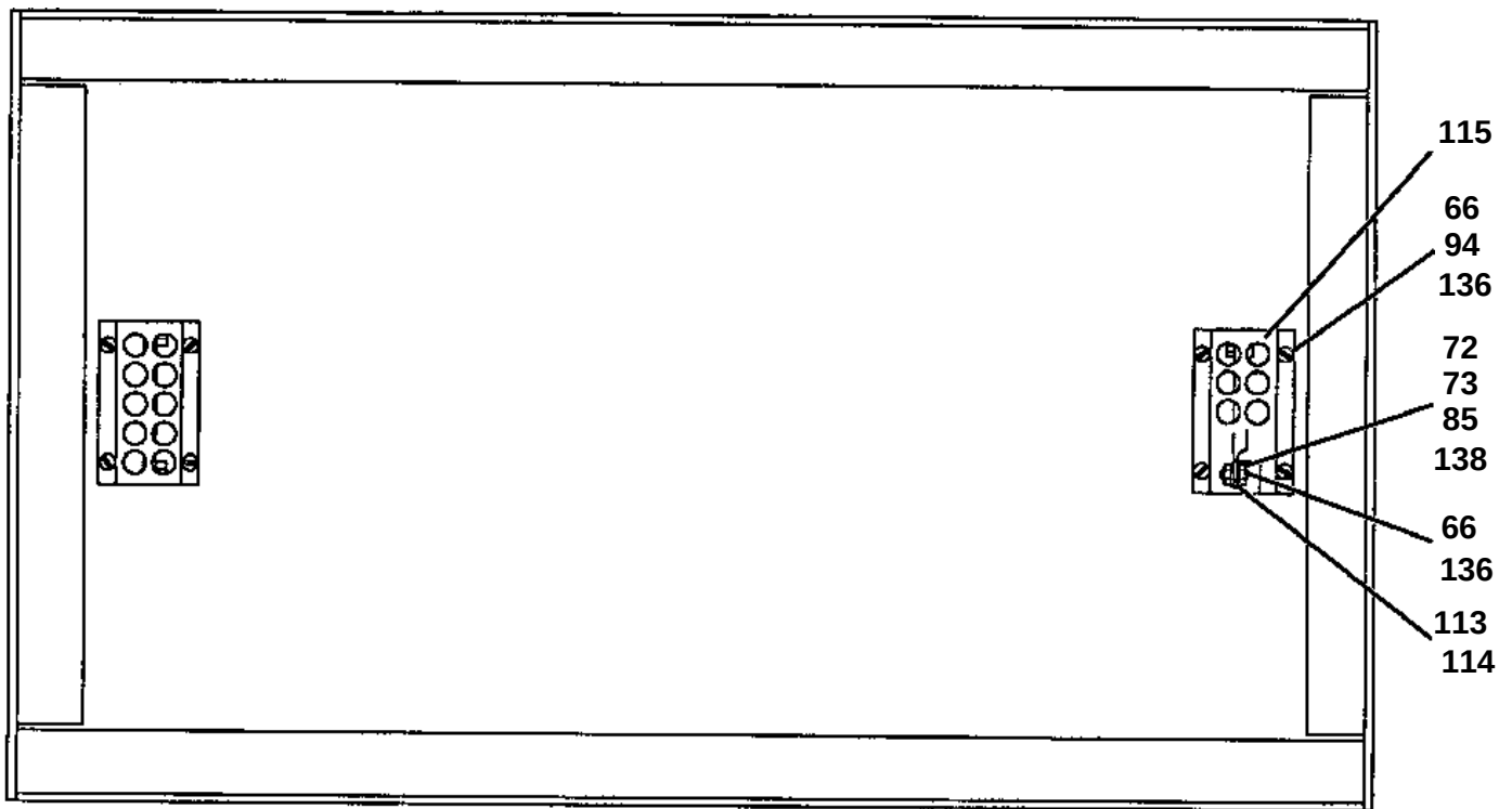
BOTTOM VIEW OF CABINET
