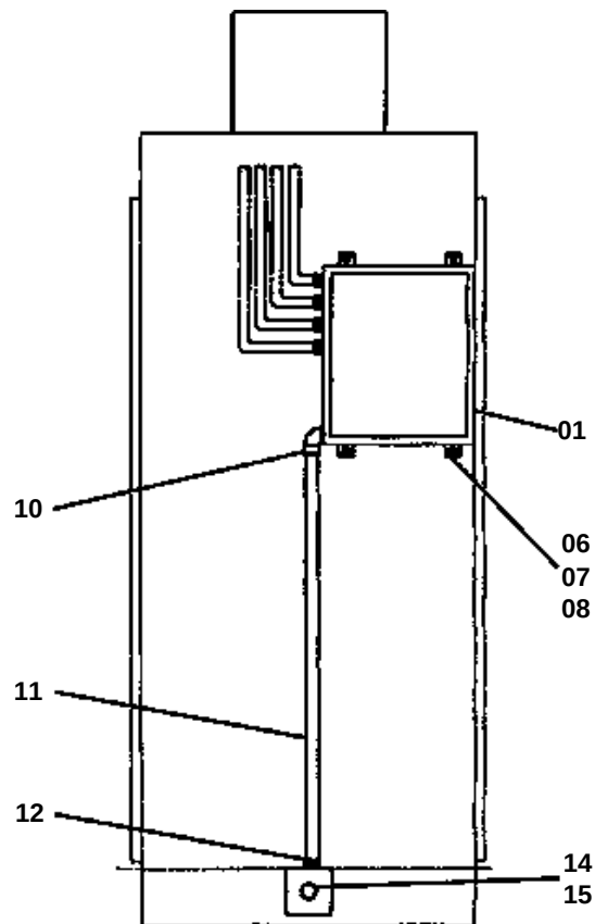
LEFT SIDE VIEW OF CONVERTER CABINET
