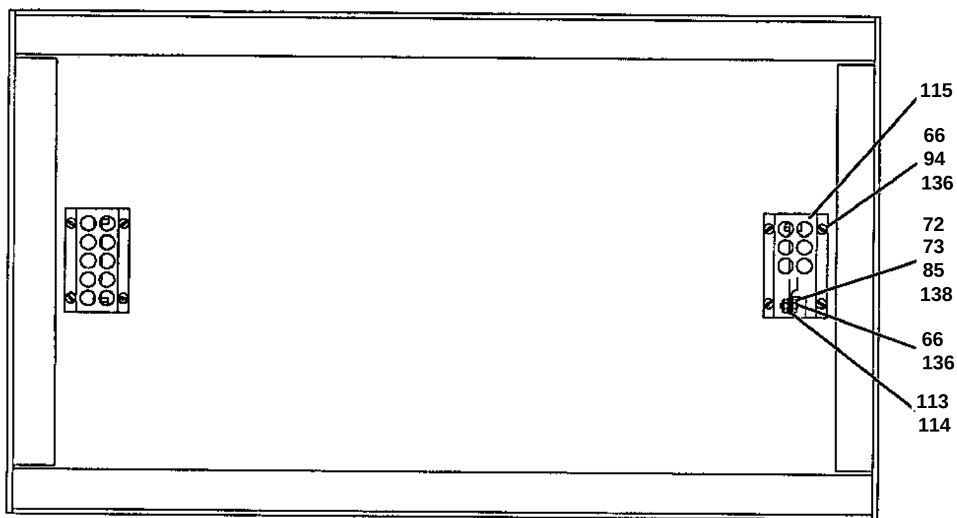
BOTTOM VIEW OF CABINET
