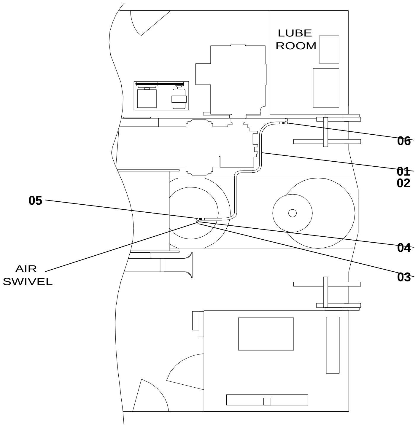
DECK PLAN
