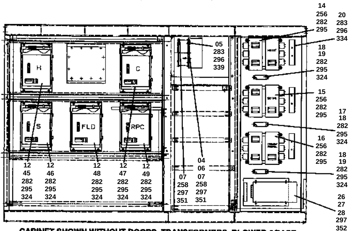
CABINET SHOWN WITHOUT DOORS, TRANSFORMERS, BLOWER & BASE
