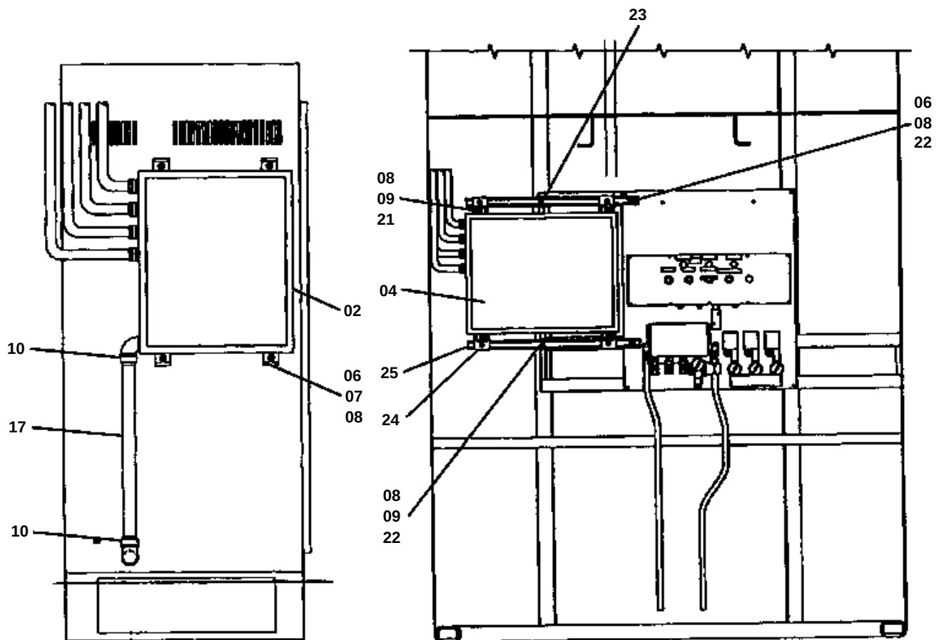
SIDE VIEW OF LUBE ROOM
