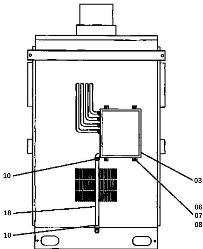
LEFT SIDE VIEW OF RPC CABINET
