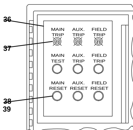
CABINET DOOR ASSEMBLY
