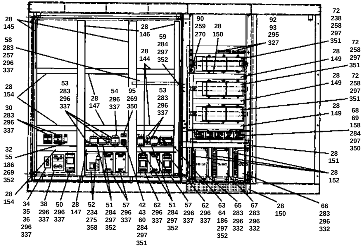
CABINET SHOWN WITHOUT DOORS, TRANSFORMERS, BLOWER & BASE
