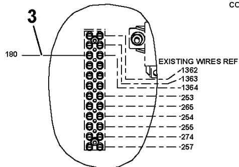
DETAIL E TERMINAL STRIP
