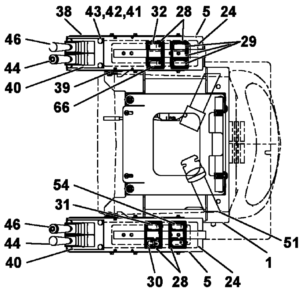
PLAN VIEW - SEAT ASSY
