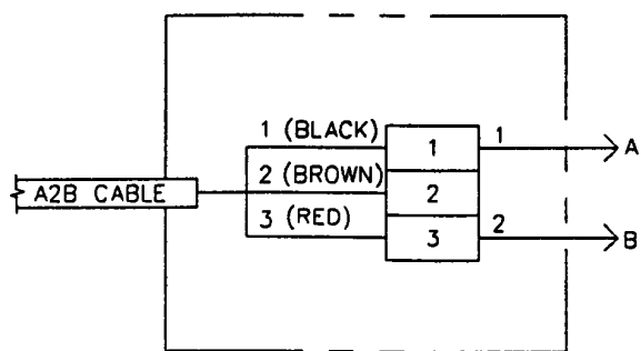
WIRING DETAIL
