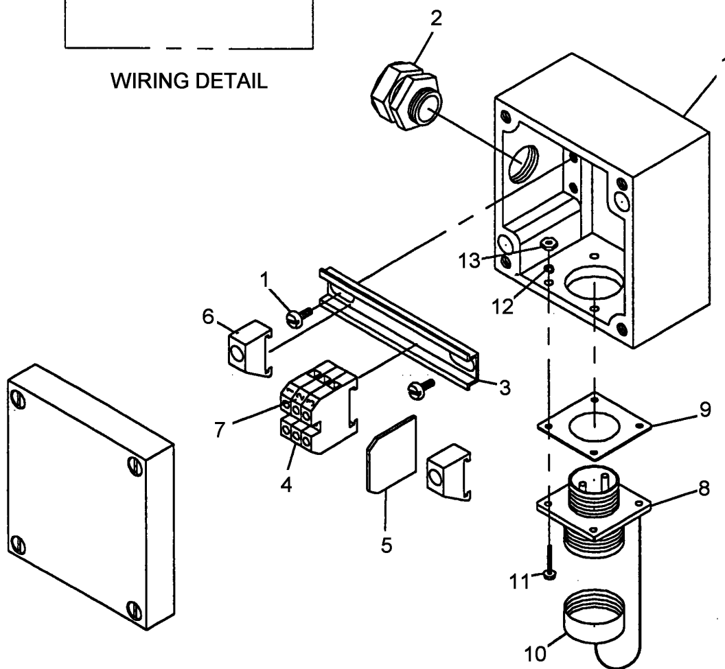
EXPLODED VIEW
