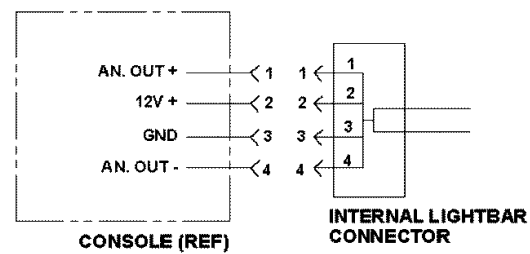
WIRING DETAIL
