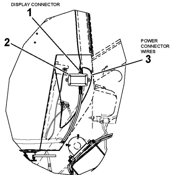
SECTION D-D CONTROL MODULE AND POWER CABLE
