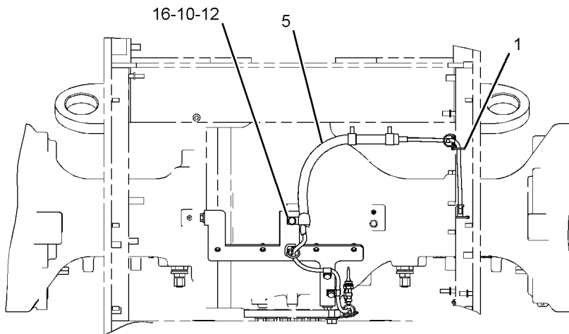
TOP VIEW (OSCILLATING AXLE)
