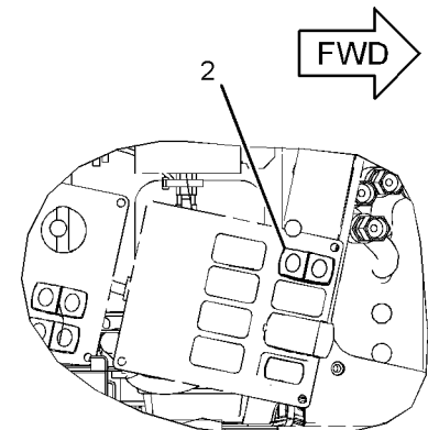
TOP VIEW (RIGHT HAND CONSOLE)
