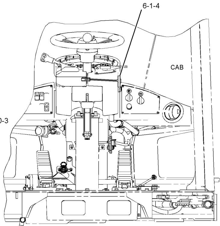
REAR VIEW
