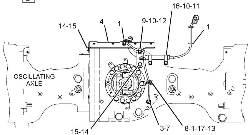
REAR VIEW
