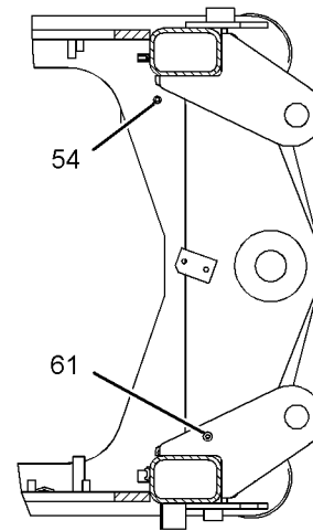
SECTION L-L
