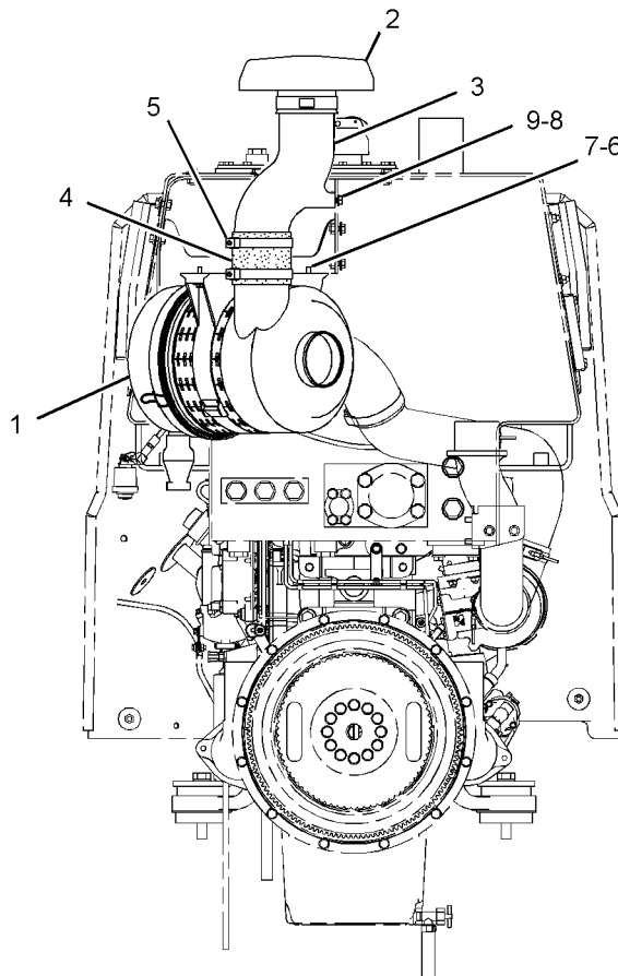
FRONT VIEW
