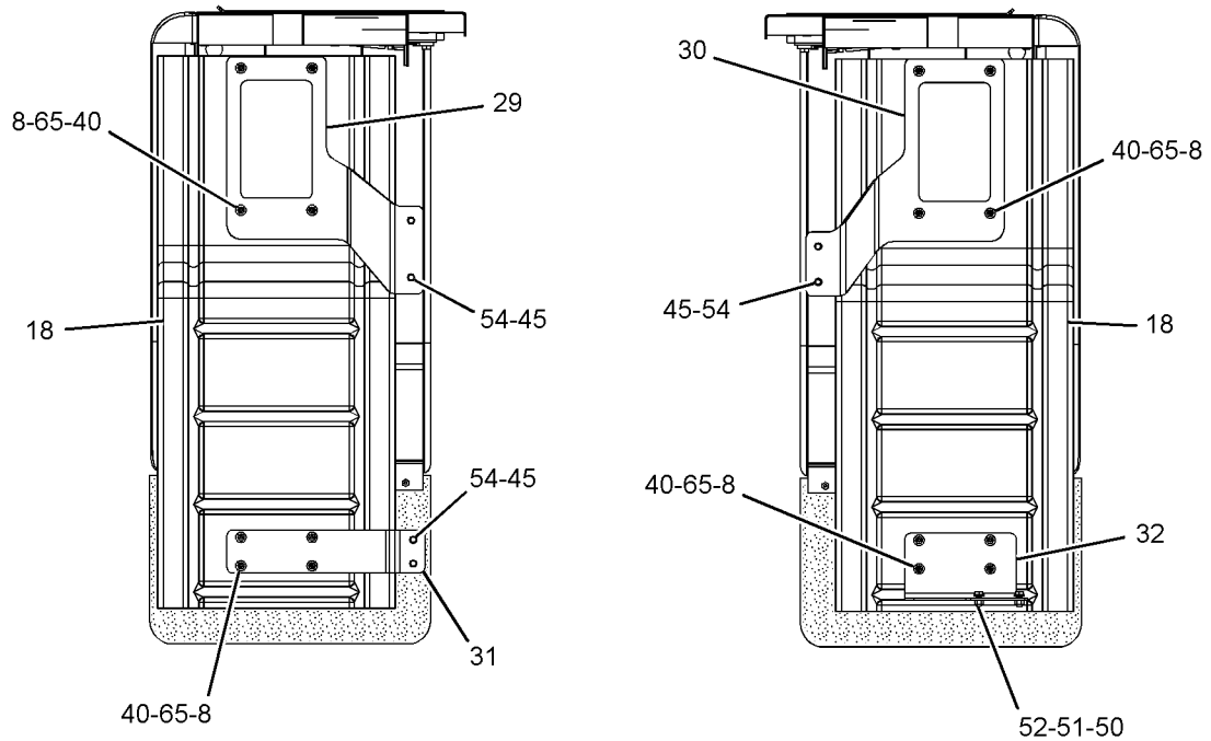
VIEW J-J
