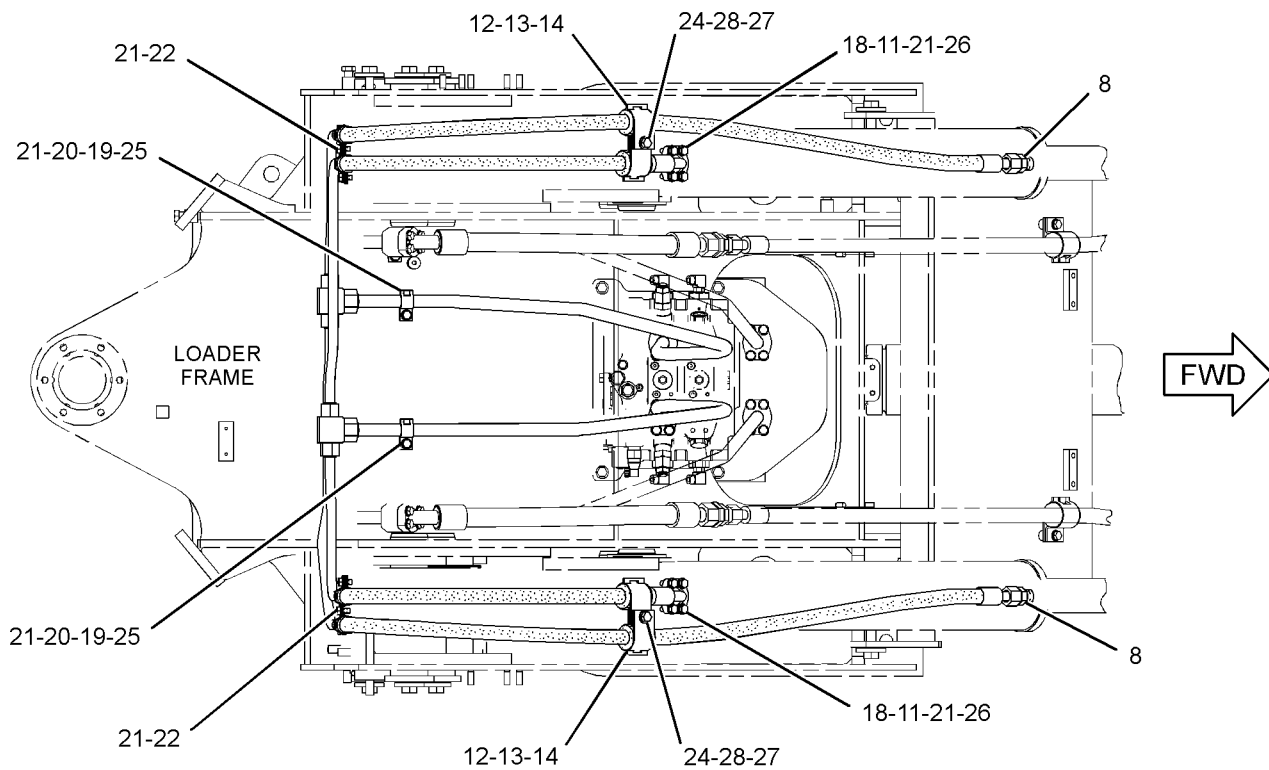
TOP VIEW
