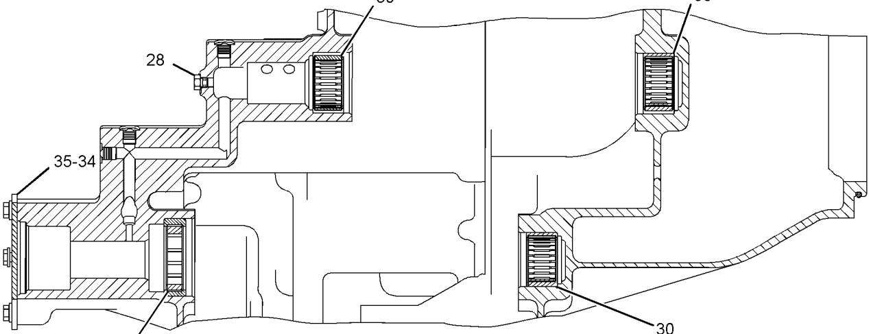
SECTION C-C
