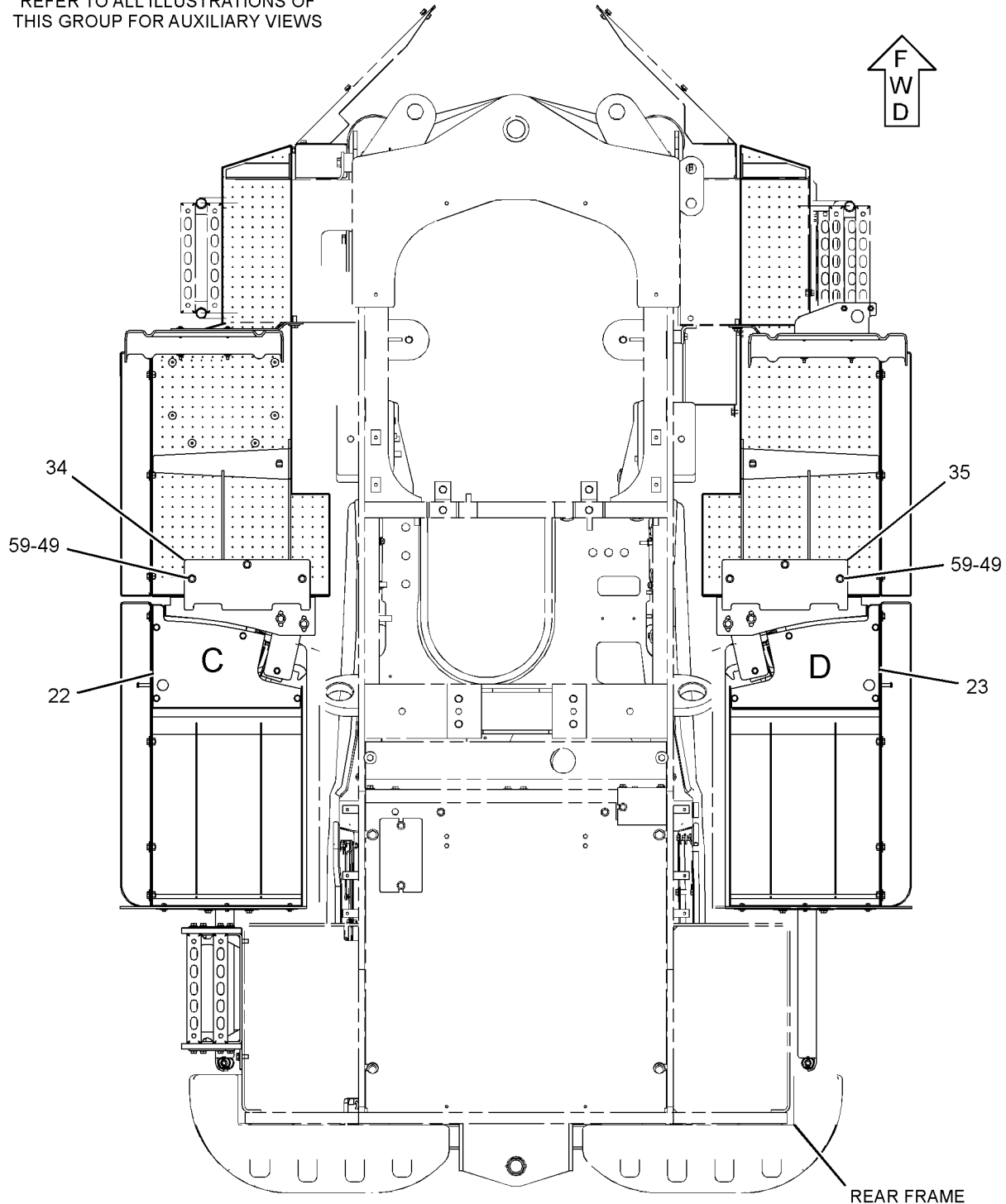
BOTTOM VIEW
