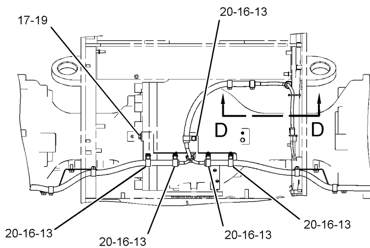
VIEW C-C
