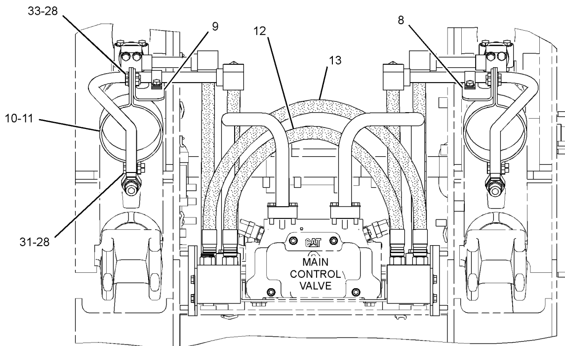
FRONT VIEW
