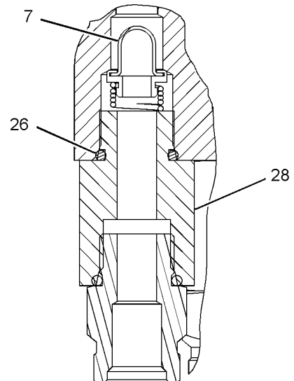
SECTION C-C
