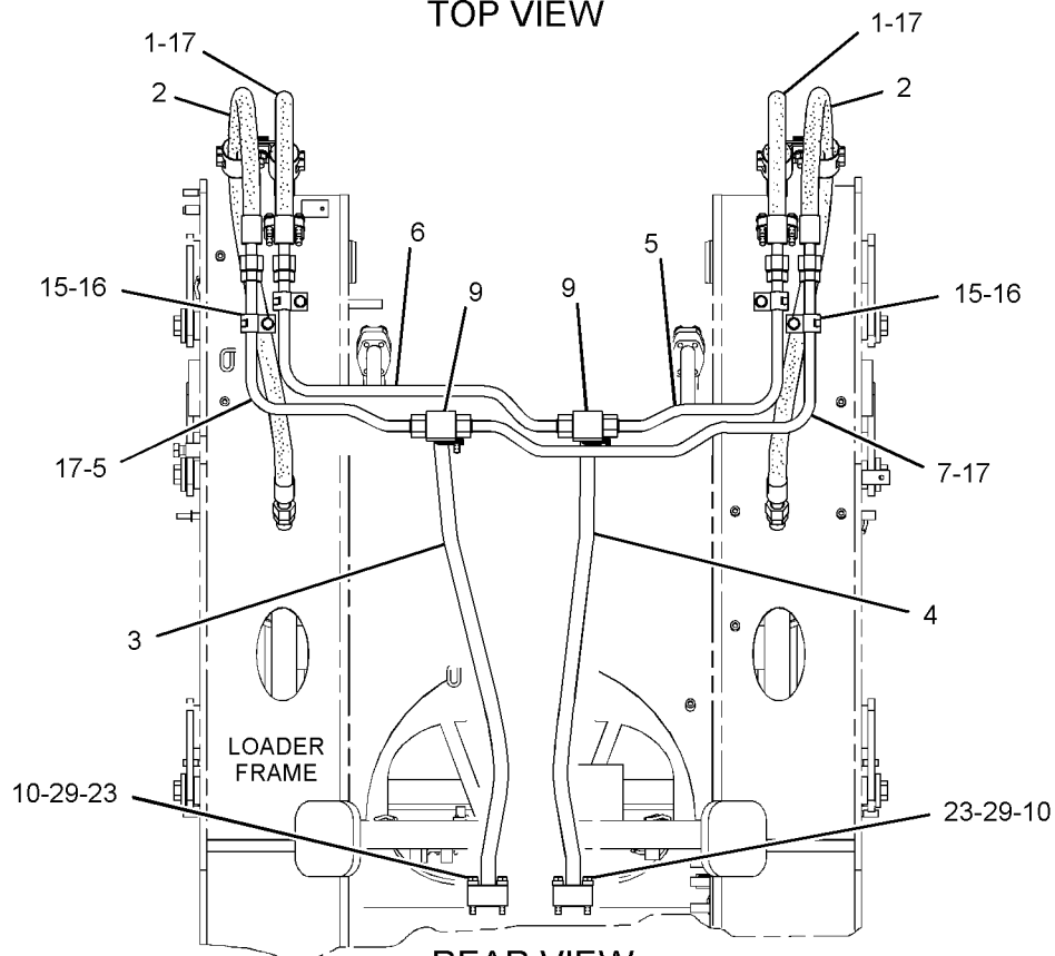
REAR VIEW
