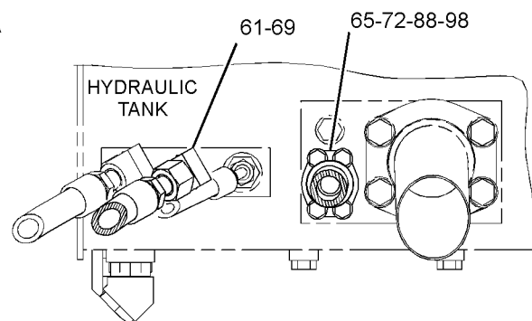
SECTION G-G
