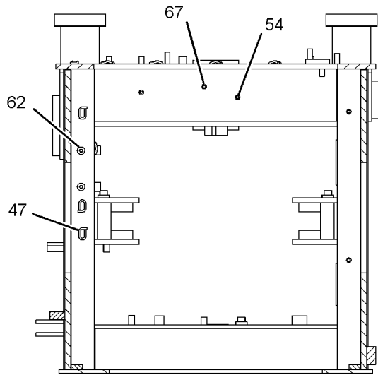
SECTION J-J
