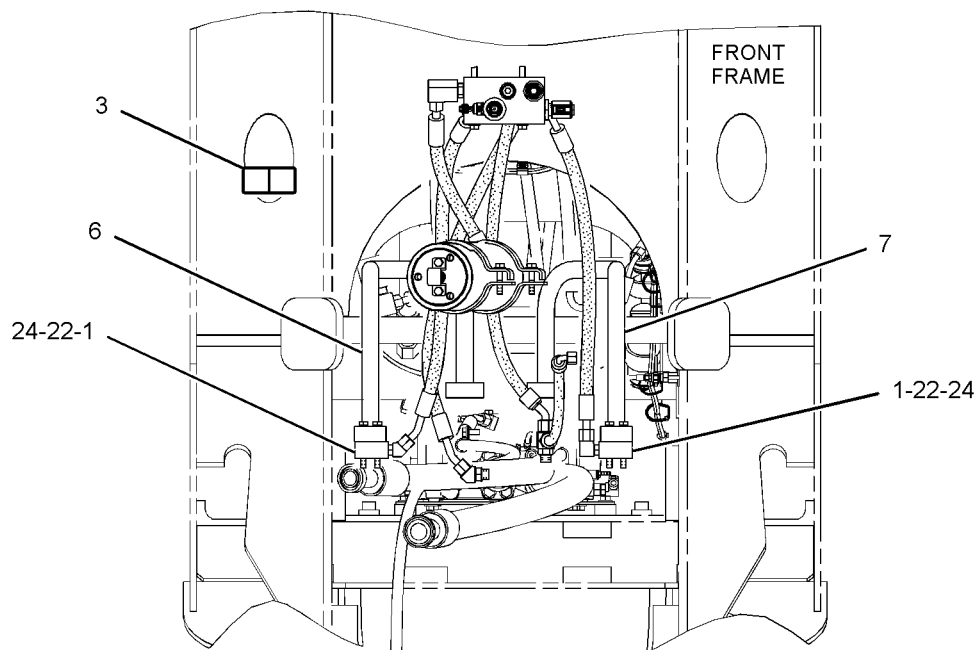
VIEW B-B
