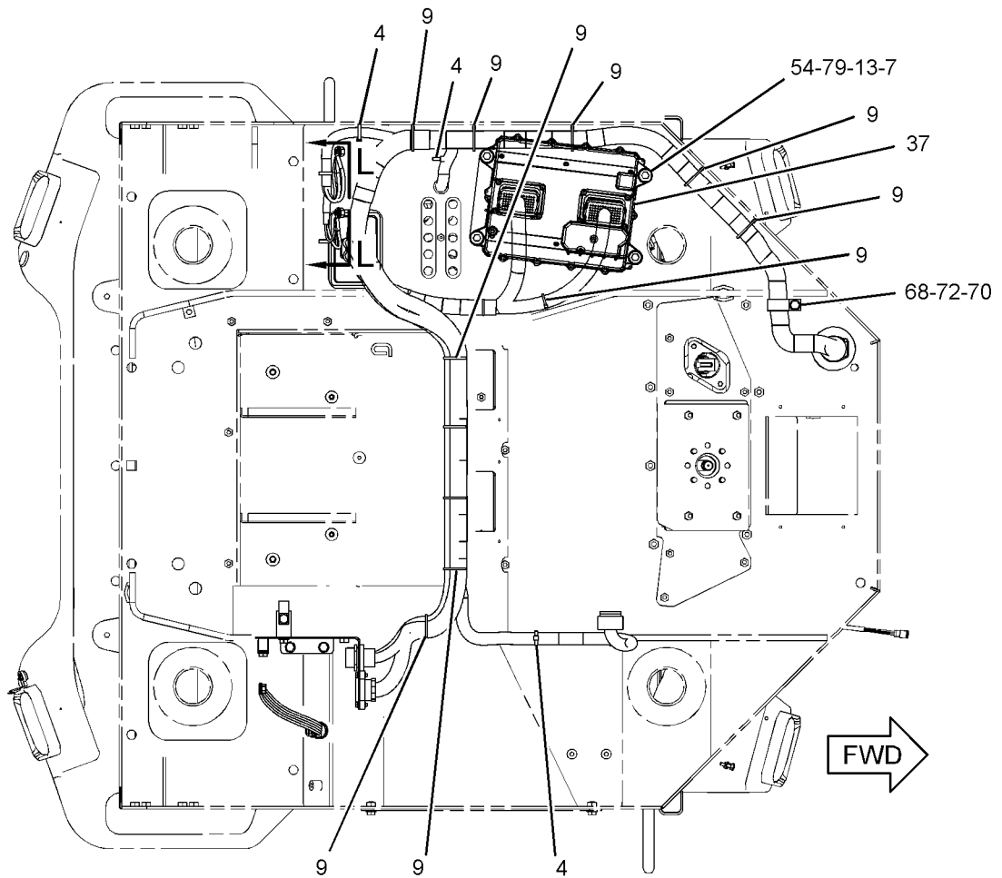
BOTTOM VIEW
