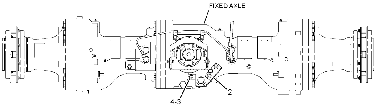
REAR VIEW
