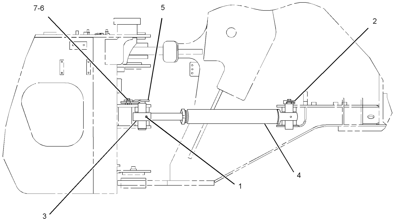
938G or IT38G RIGHT SIDE VIEW
