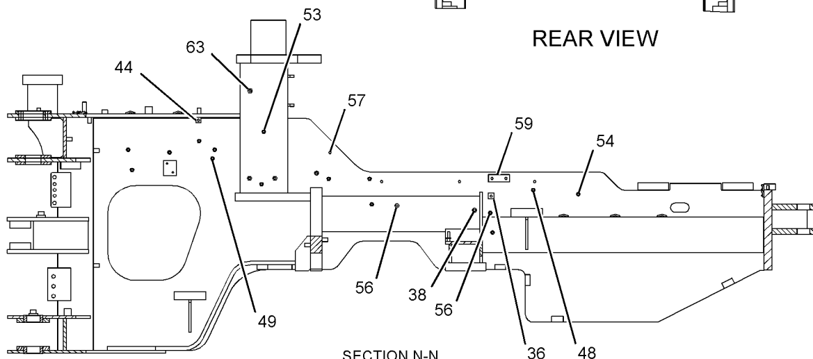
SECTION N-N
