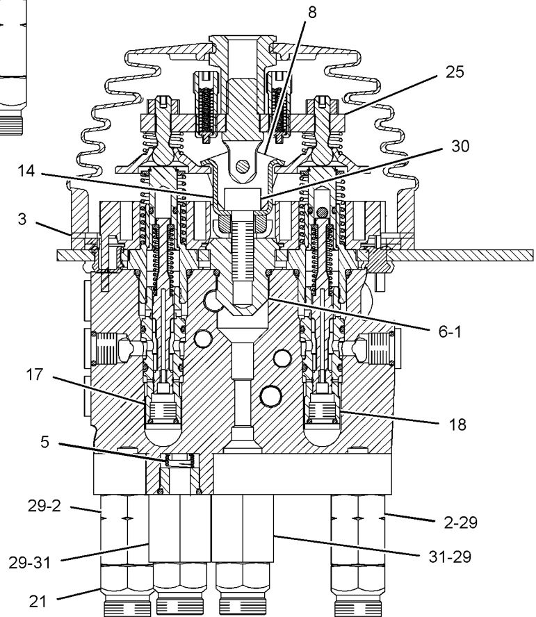
SECTION C-C
