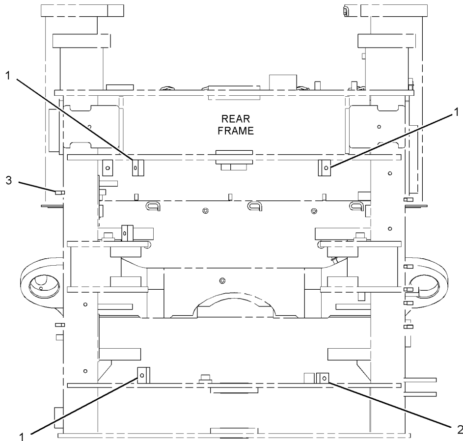
FRONT VIEW
