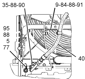
VIEW B-B
