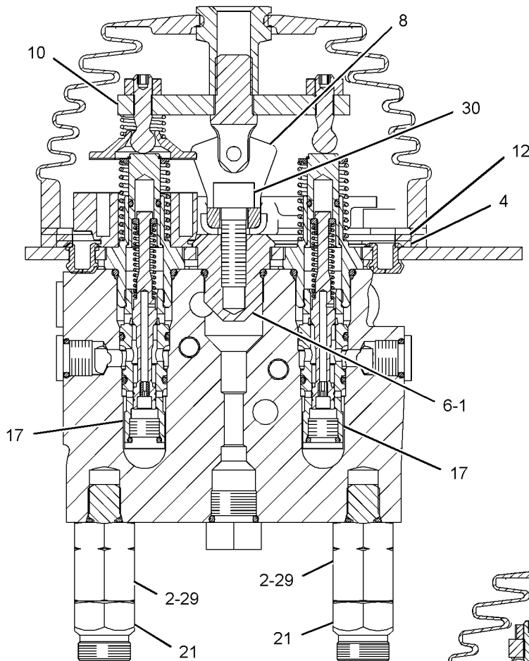
SECTION B-B
