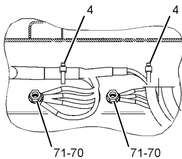
VIEW L-L
