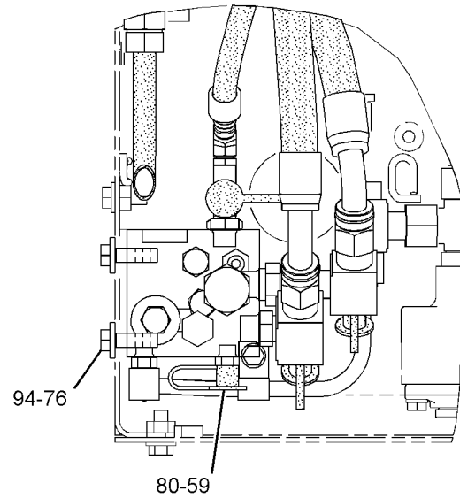
SECTION H-H
