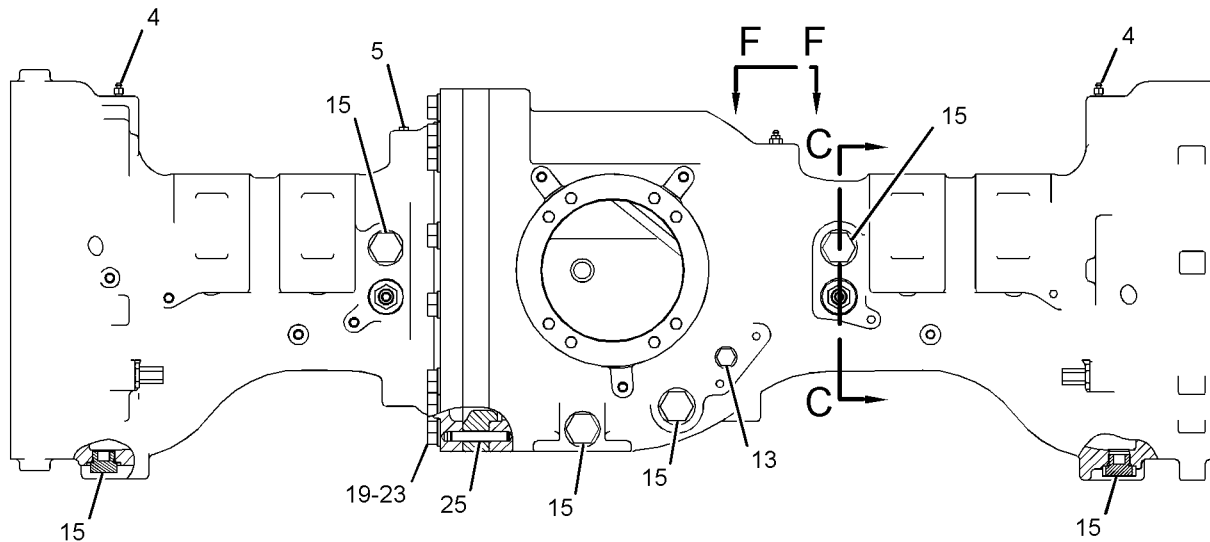
REAR VIEW
