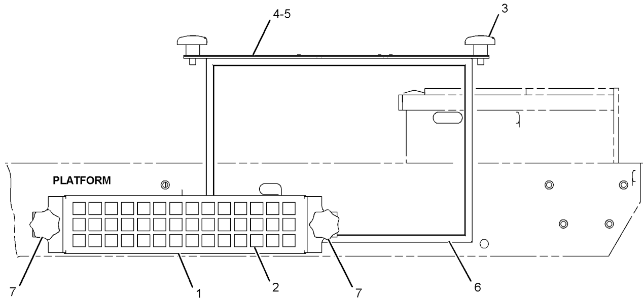
LEFT SIDE VIEW <END>
