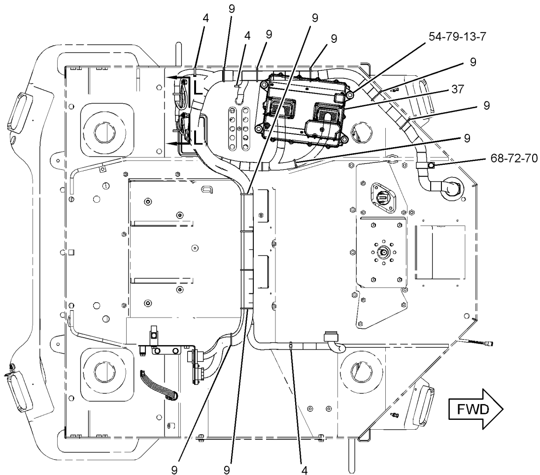
BOTTOM VIEW
