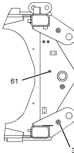
SECTION K-K
