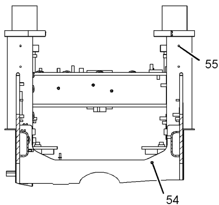
SECTION G-G
