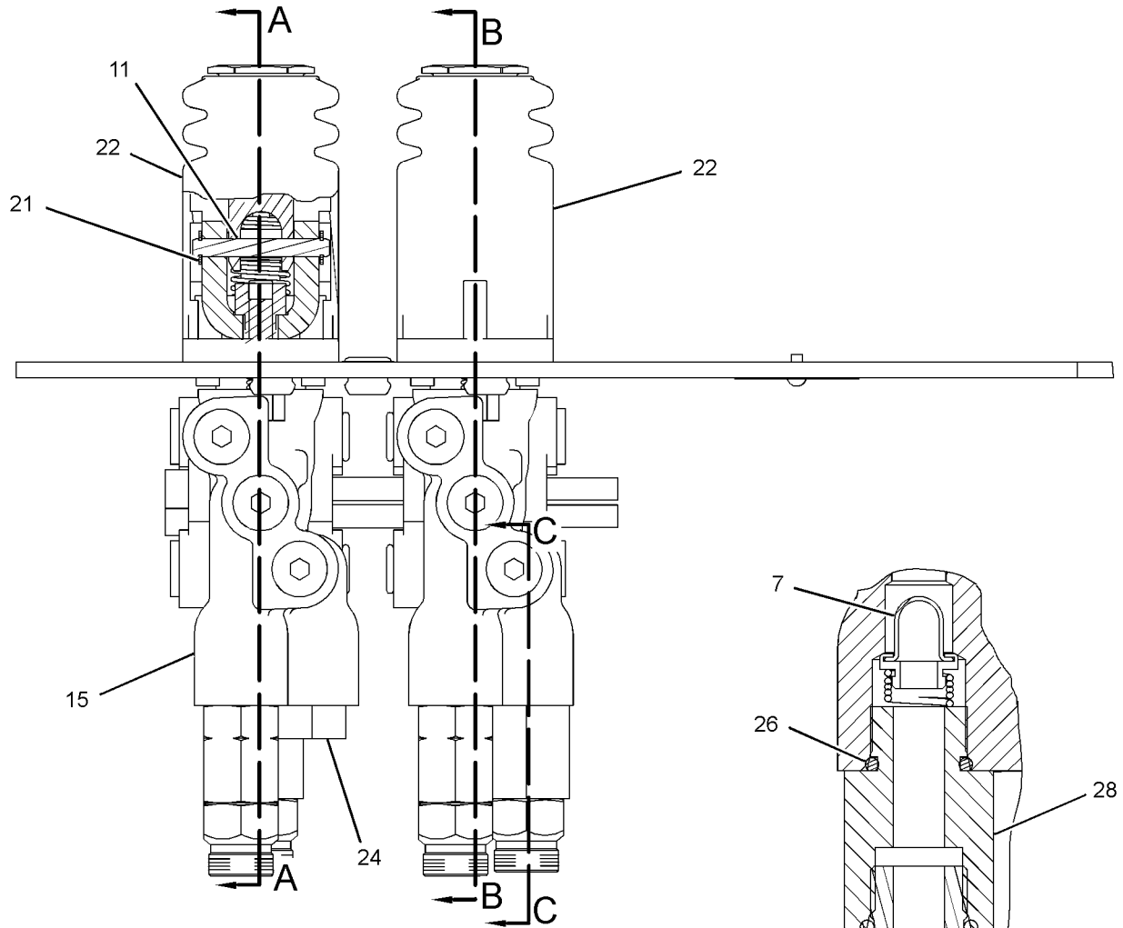
REAR VIEW
