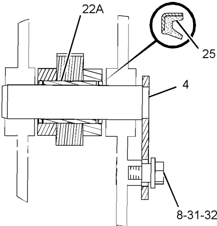
SECTION L-L
