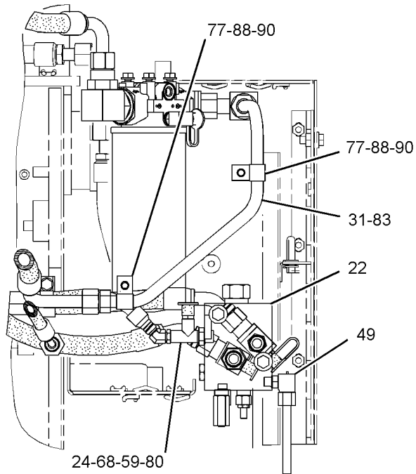
SECTION F-F
