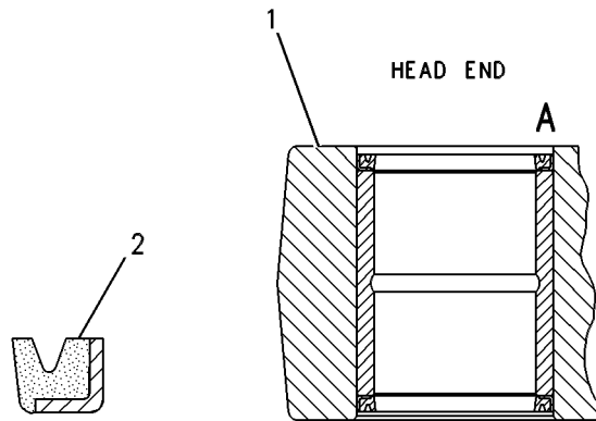
CYLINDER ASSEMBLY
