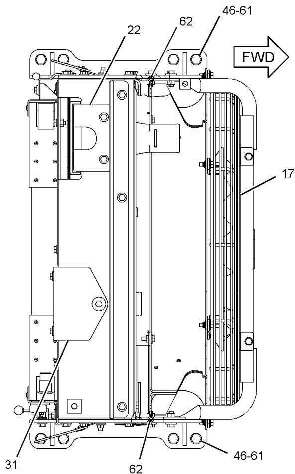
TOP VIEW
