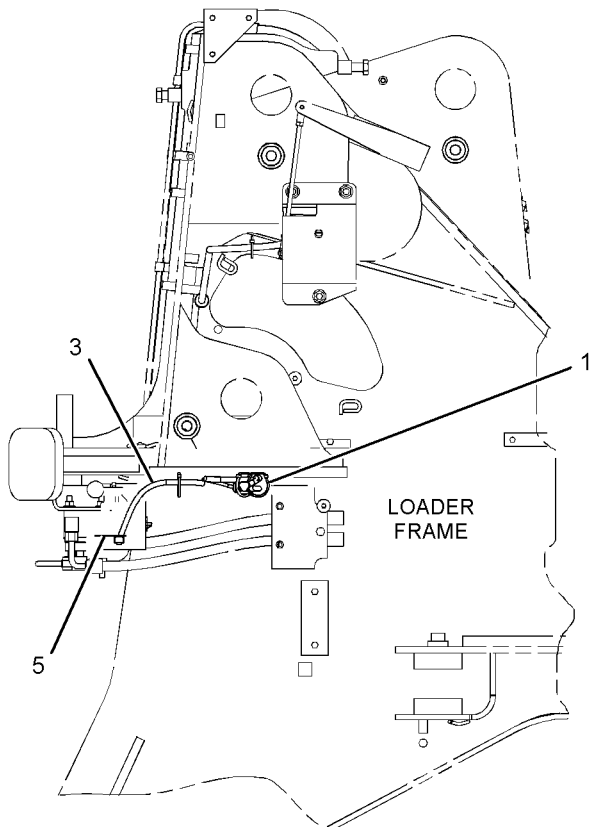
RIGHT SIDE VIEW (OF LOADER FRAME)
