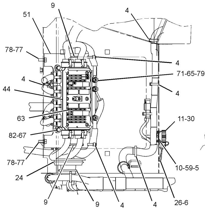
VIEW D-D
