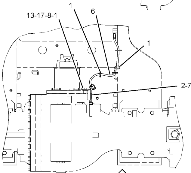
BOTTOM VIEW (FIXED AXLE)
