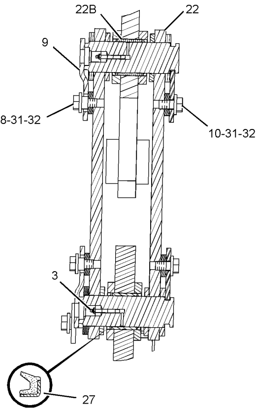
SECTION J-J
