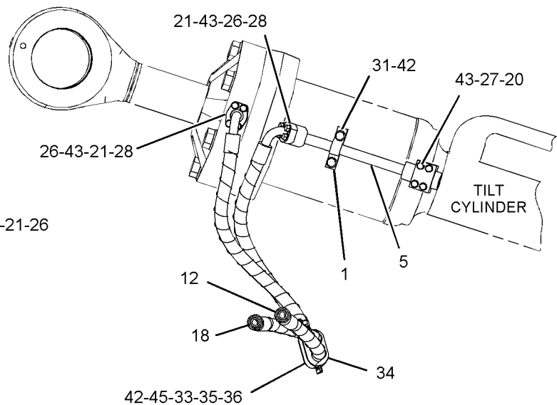
VIEW F-F (GUARD REMOVED)
