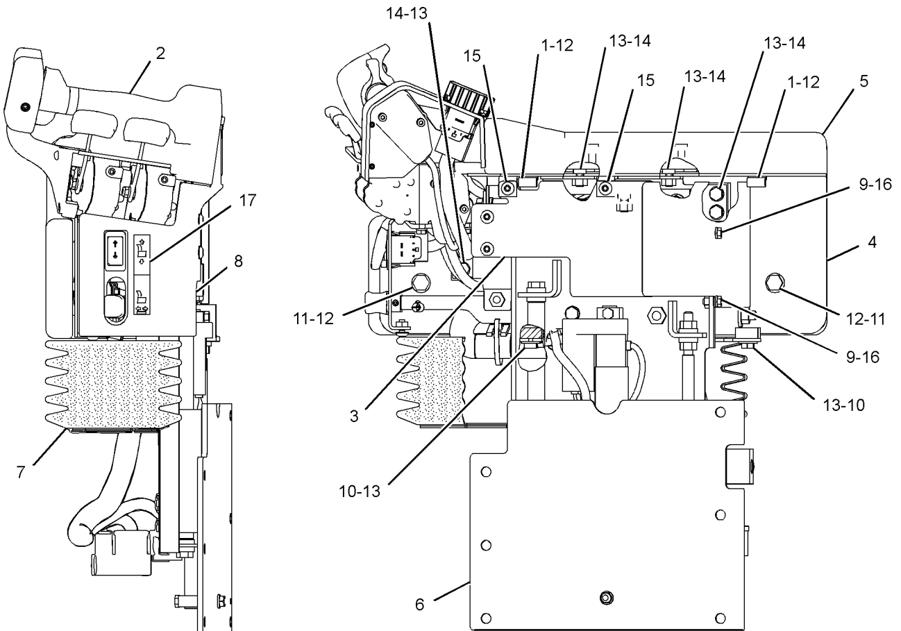
FRONT VIEW
