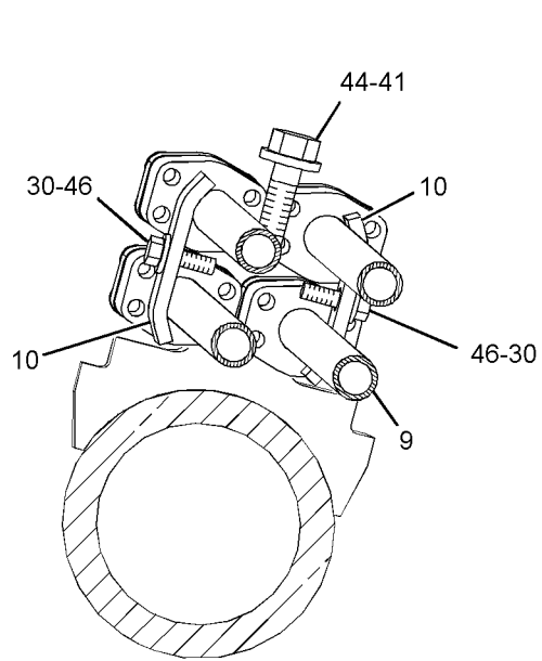
SECTION C-C (GUARD REMOVED)
