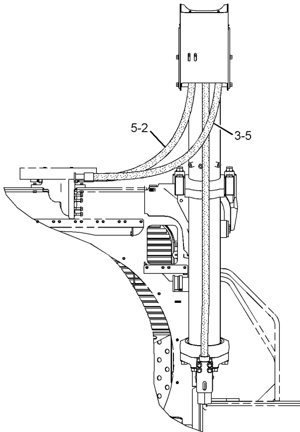
REAR VIEW
