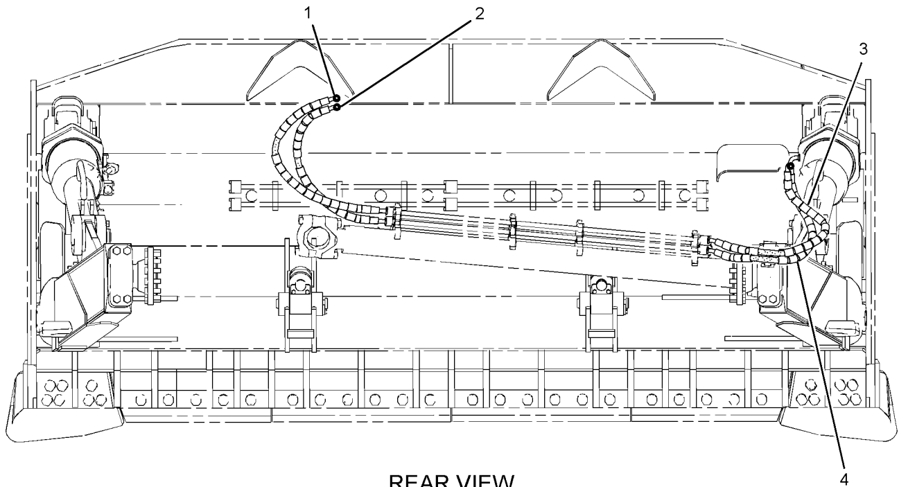
REAR VIEW
