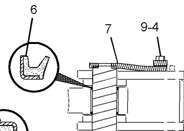
VIEW E-E
