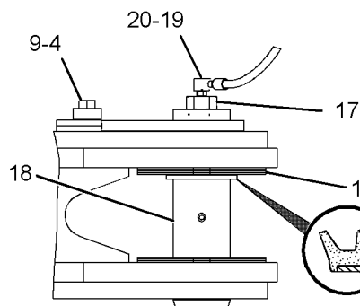
VIEW D-D
