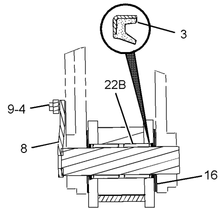
VIEW C-C
