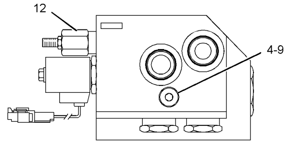
VIEW B-B
