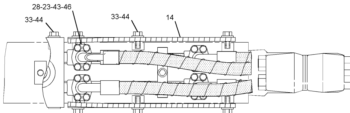
SECTION E-E
