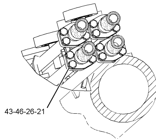
SECTION B-B (GUARD REMOVED)
