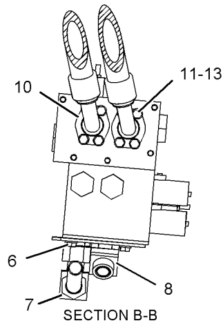
SECTION B-B
