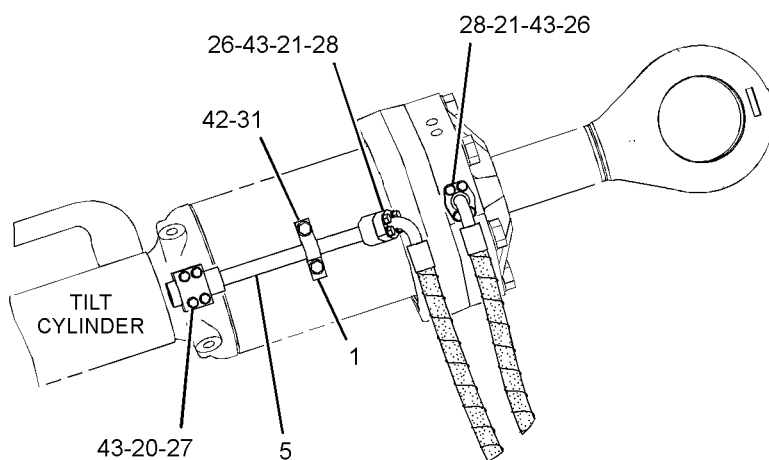
VIEW A-A (GUARD REMOVED)
