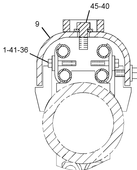
SECTION C-C
