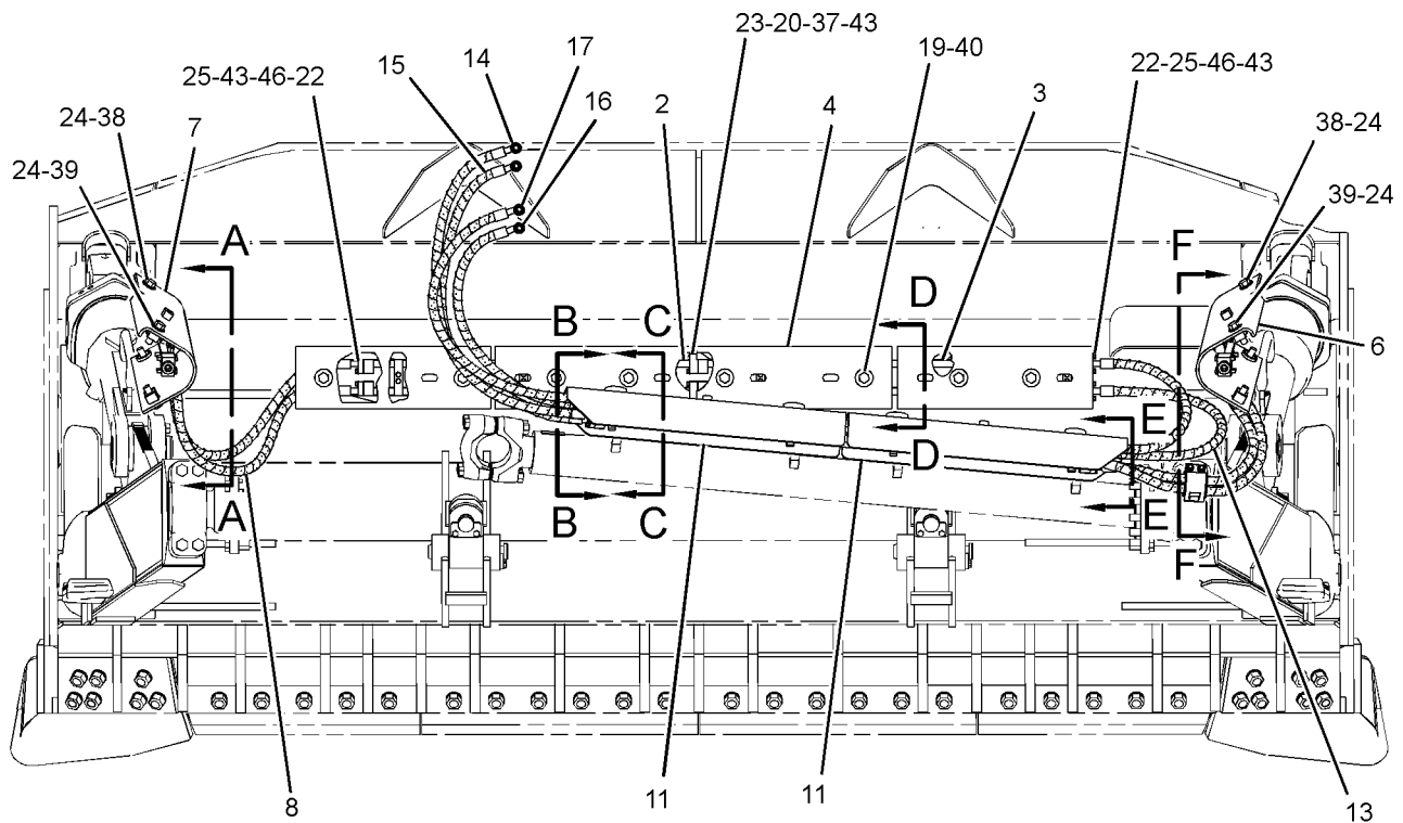
REAR VIEW
