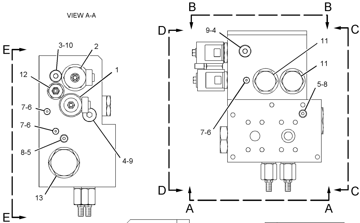
VIEW D-D
