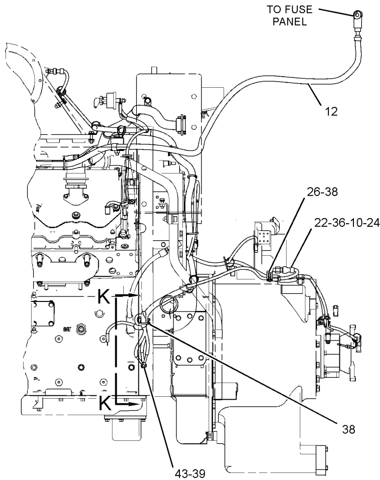
LEFT SIDE VIEW OF ENGINE
