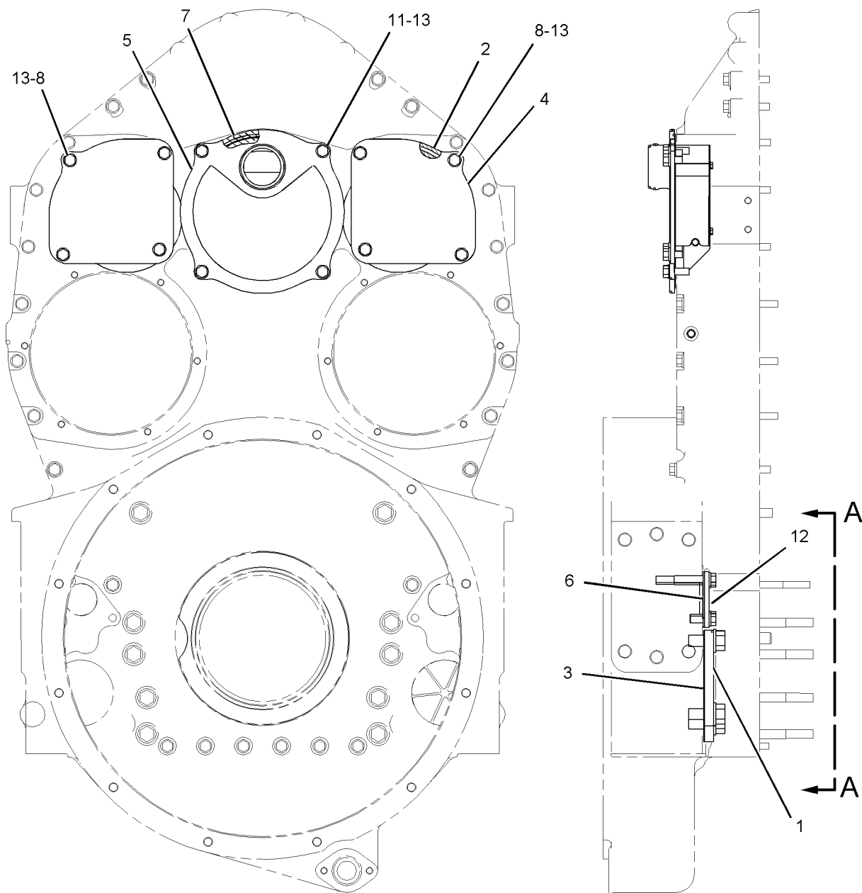
FRONT VIEW
