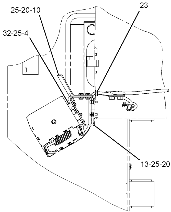
VIEW D-D
