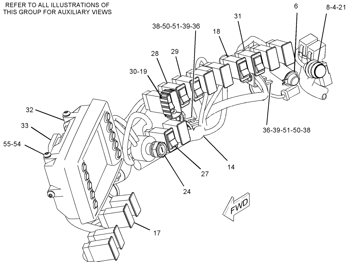
VIEW OF AREA D
