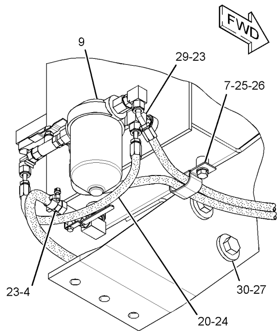
(COVER AND LATCH REMOVED FOR CLARITY)
