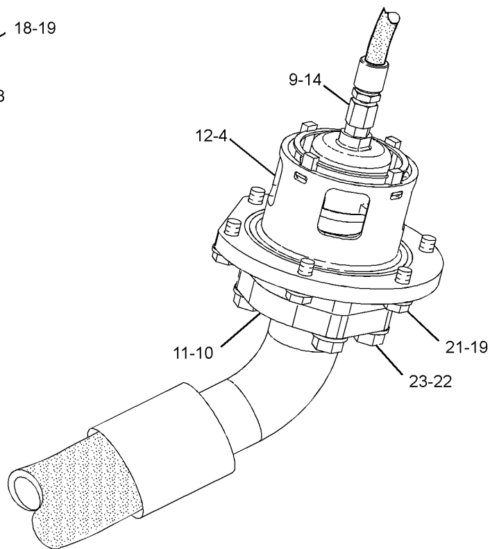
VIEW OF AREA B
