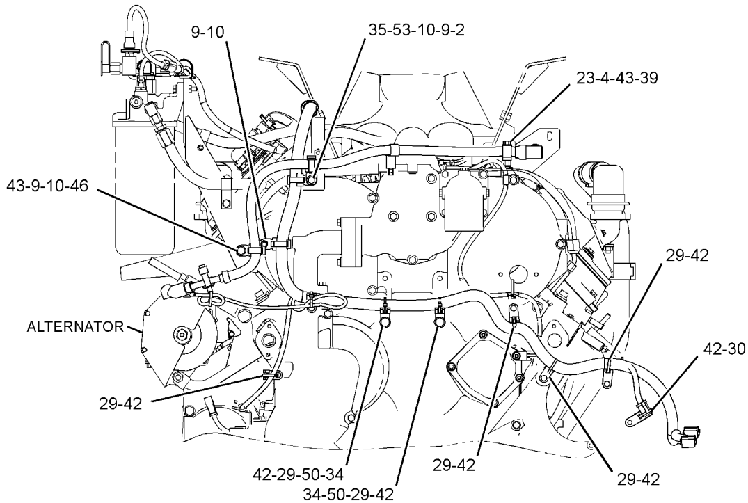
FRONT VIEW OF ENGINE
