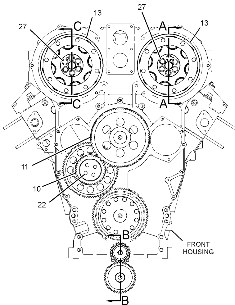
FRONT VIEW OF ENGINE
