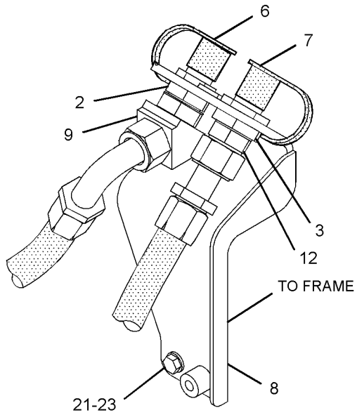
VIEW OF AREA B
