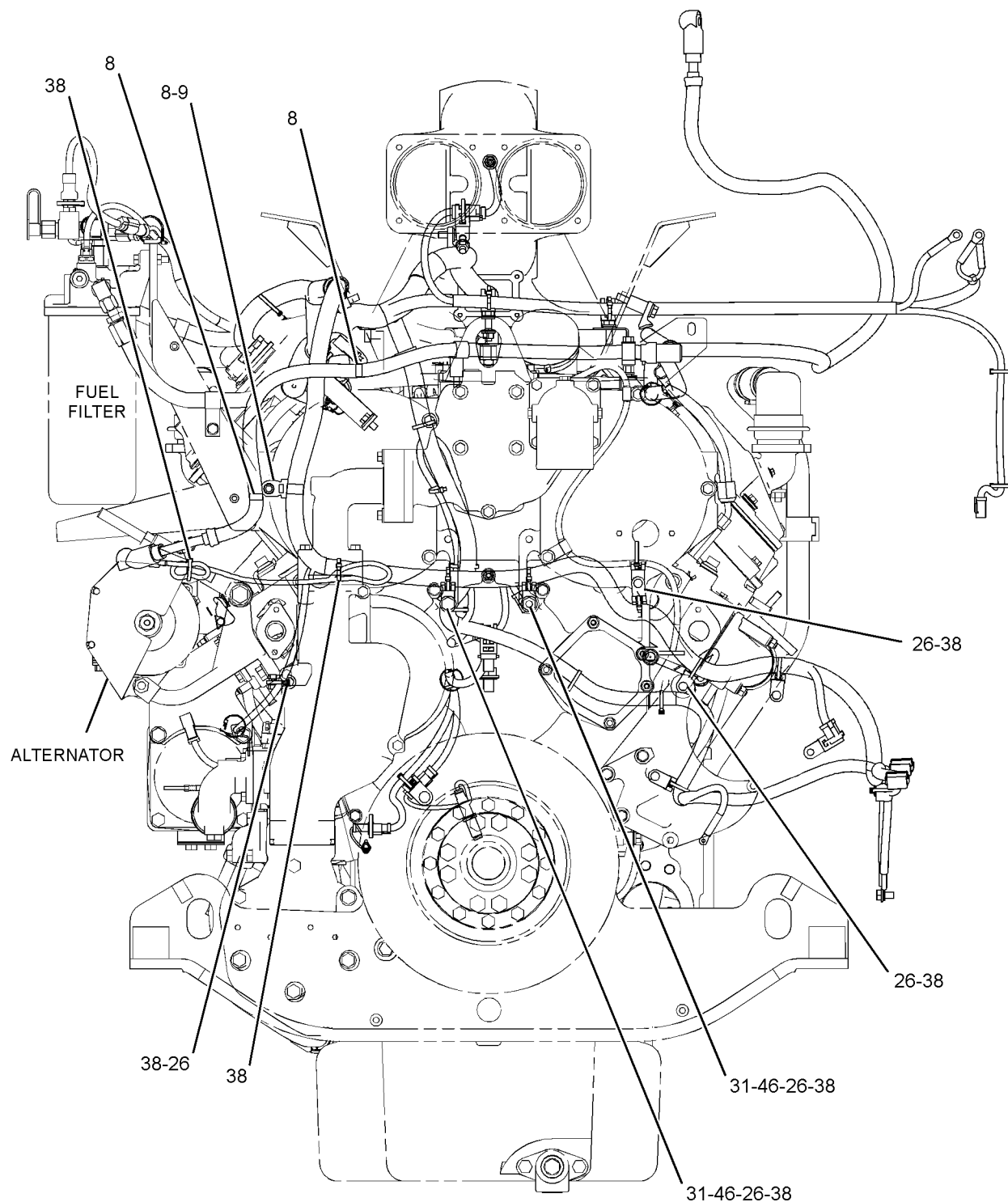
FRONT VIEW OF ENGINE
