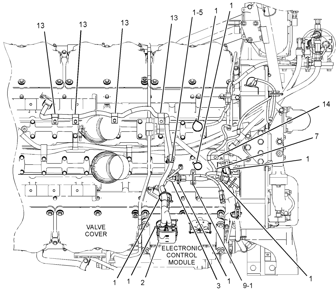
TOP VIEW OF ENGINE
