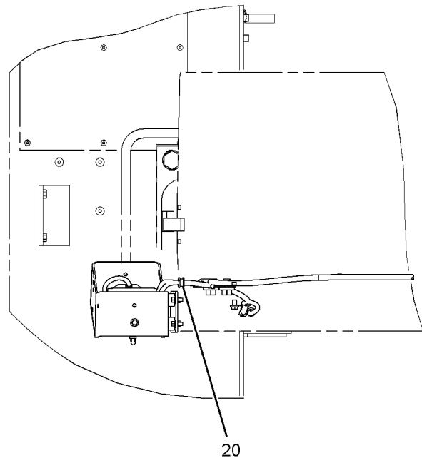
VIEW D-D
