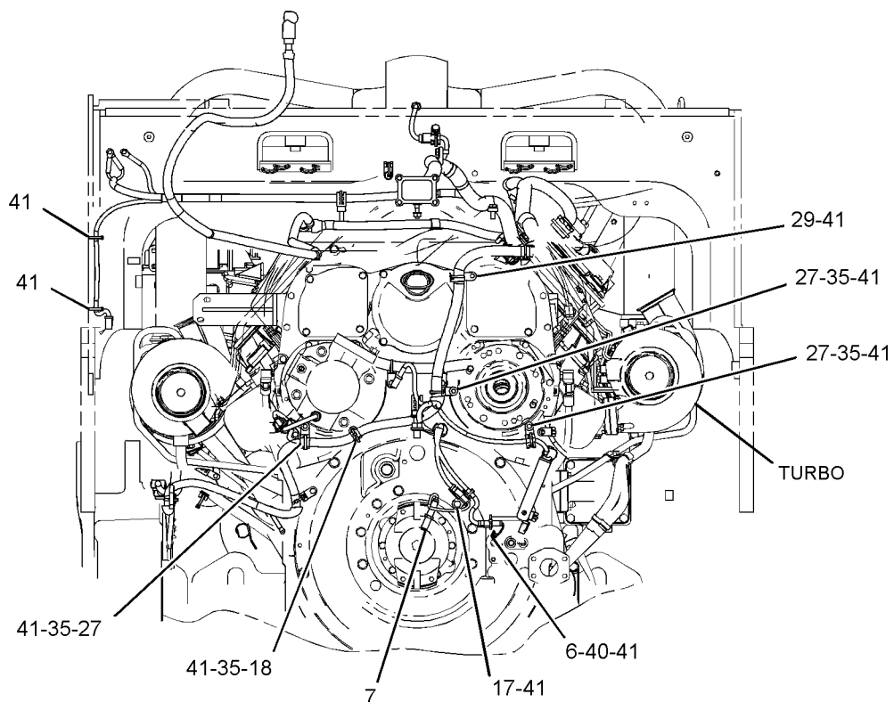
REAR VIEW OF ENGINE
