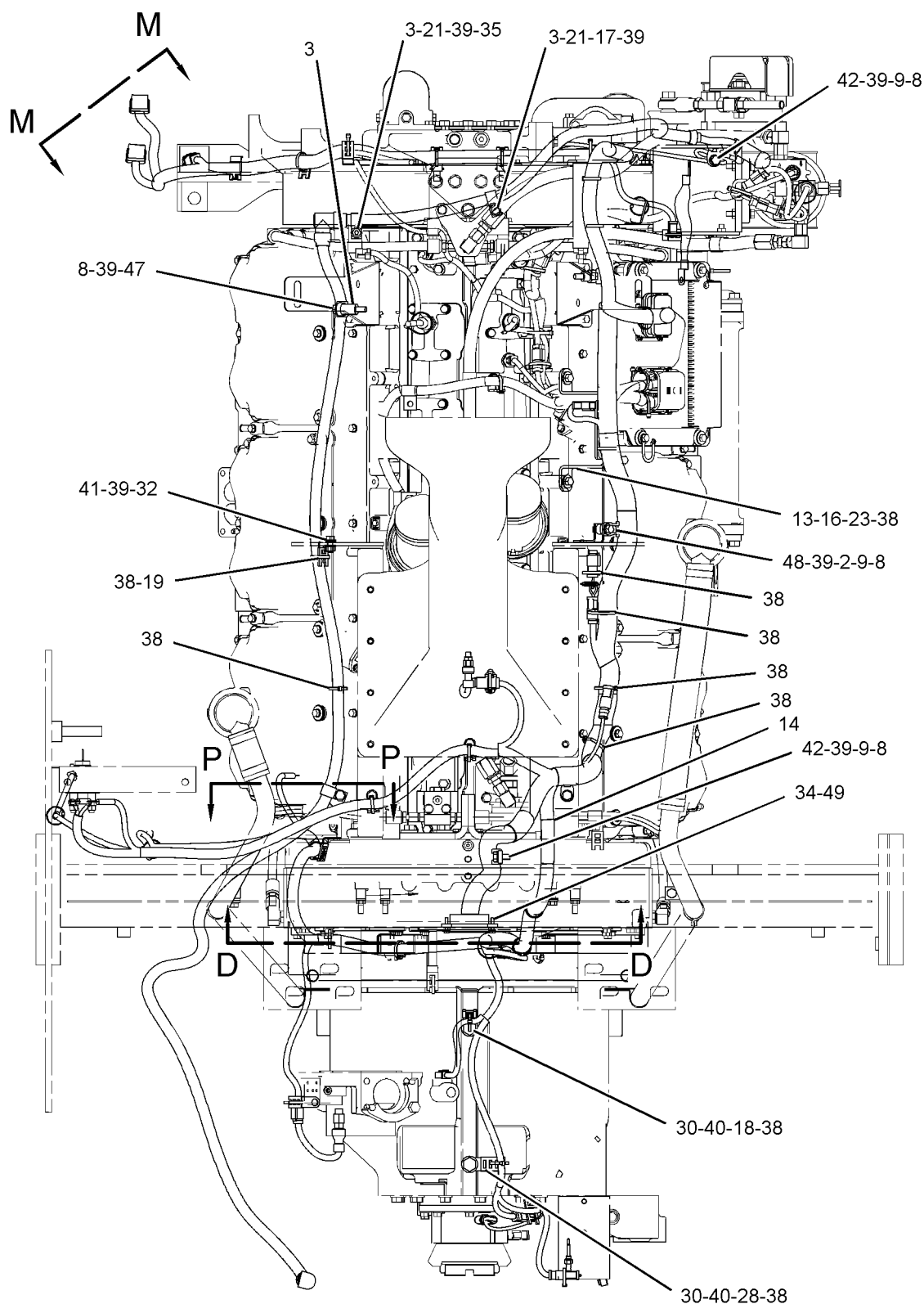
TOP VIEW OF ENGINE
