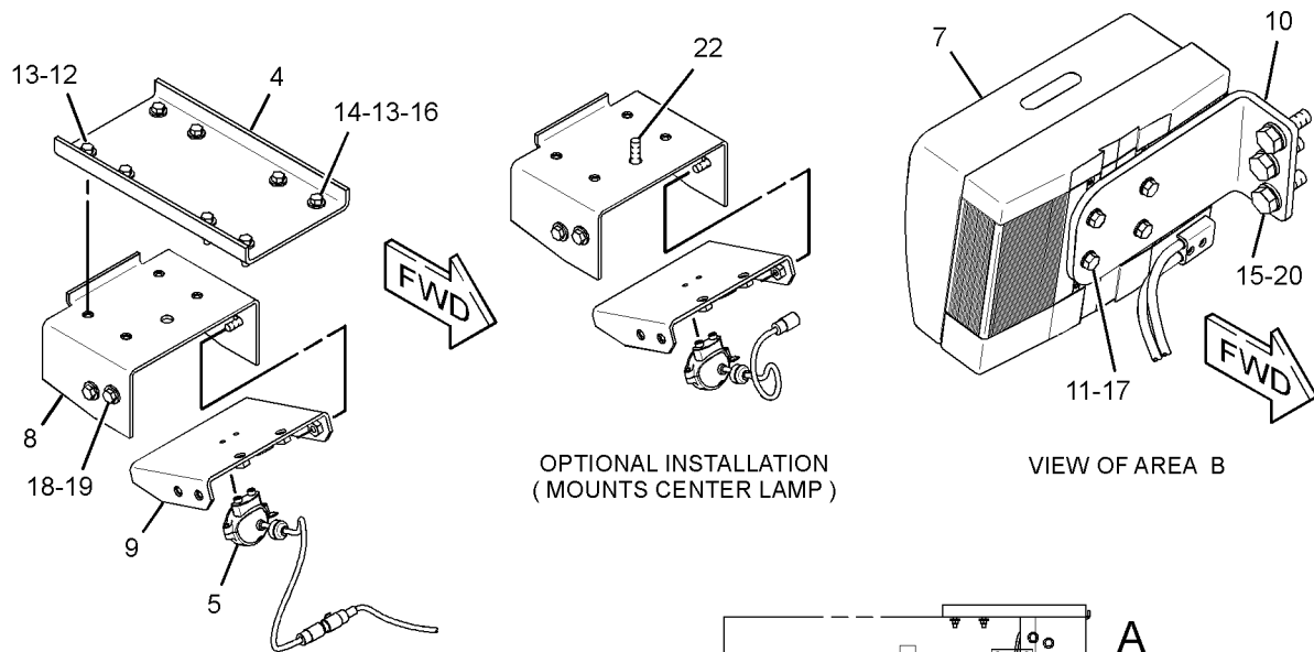
VIEW OF AREA A (EXPLODED)
