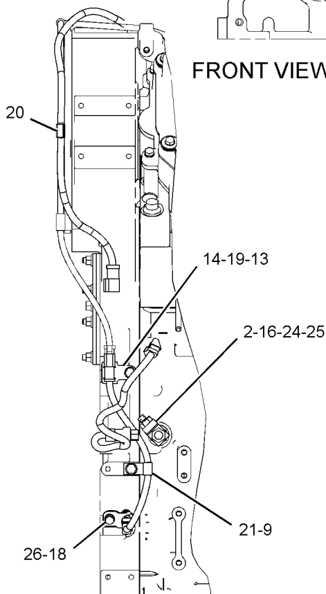
LEFT SIDE VIEW OF ENGINE
