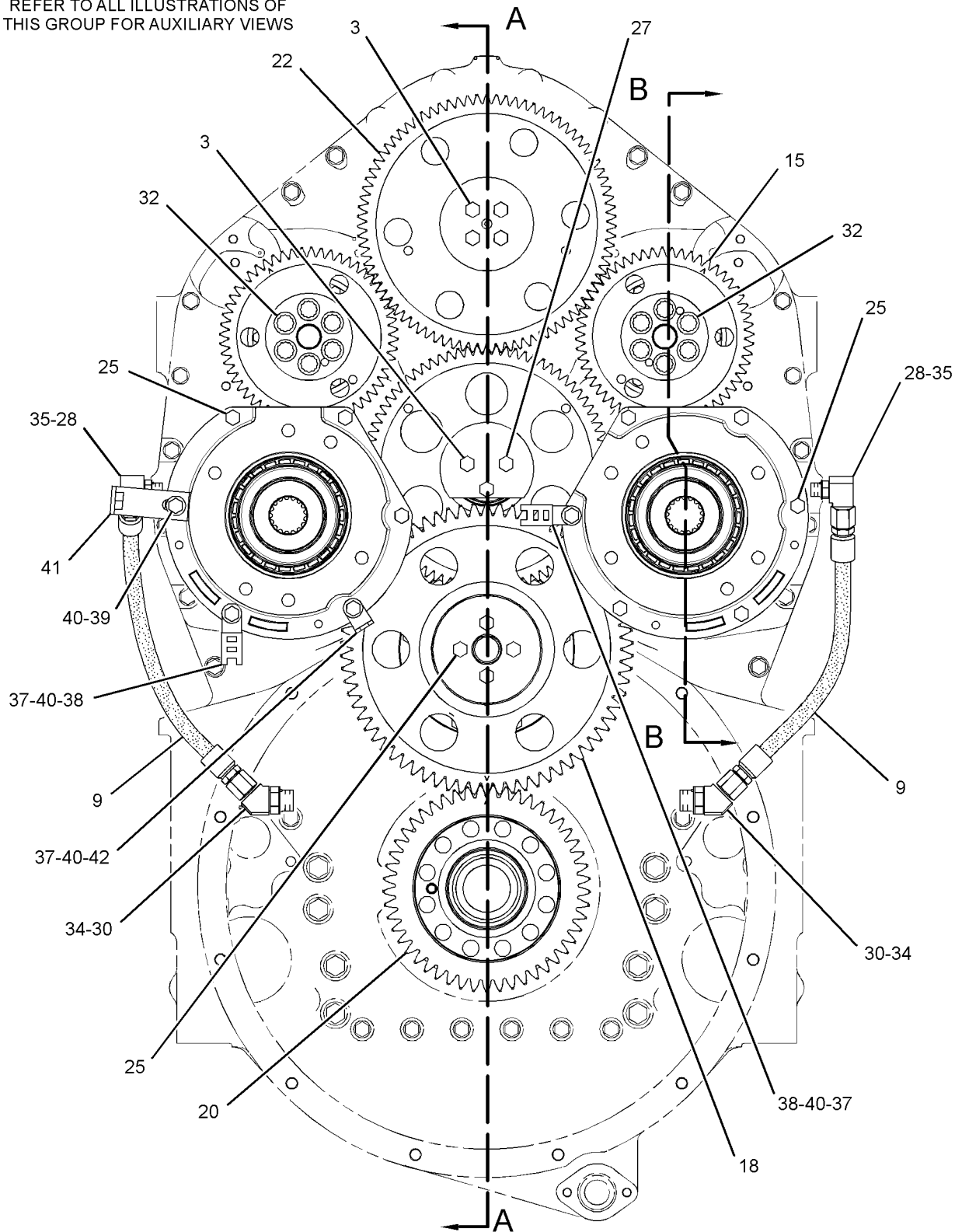
REAR VIEW OF THE ENGINE
