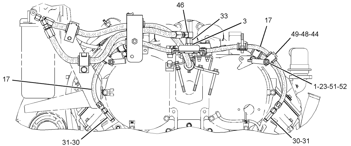
FRONT VIEW OF ENGINE
