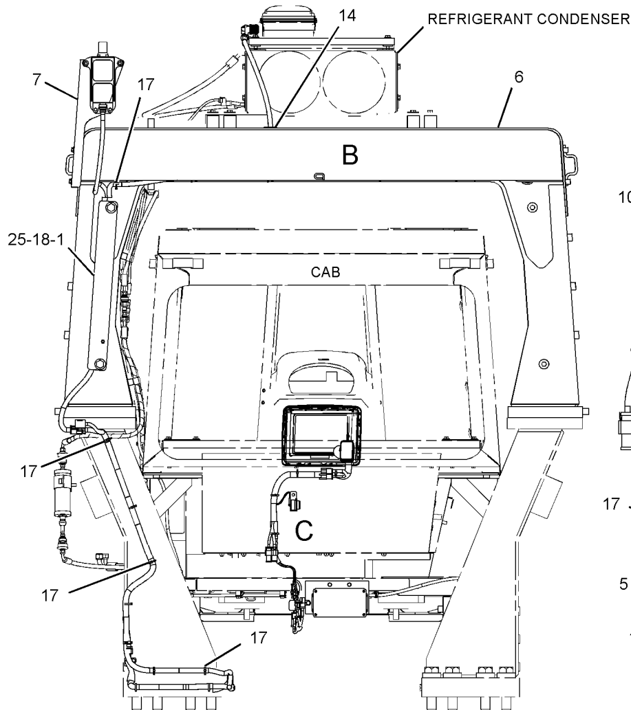
REAR VIEW
