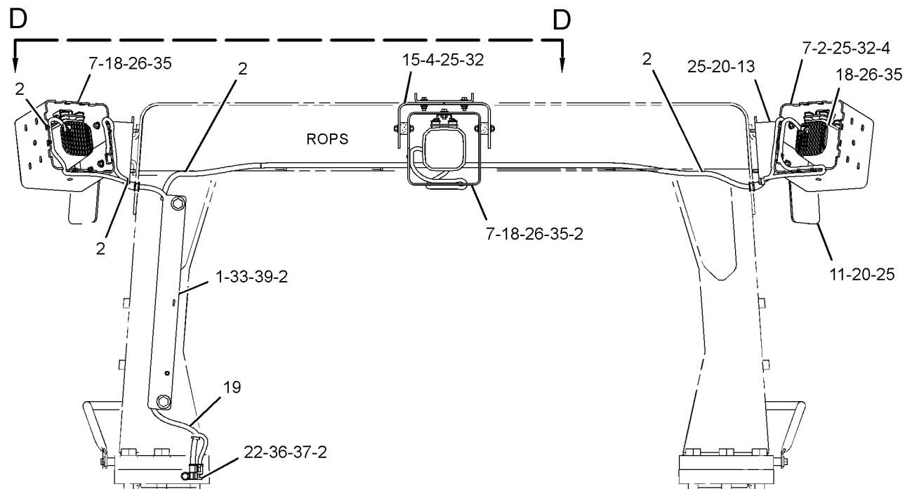
REAR VIEW
