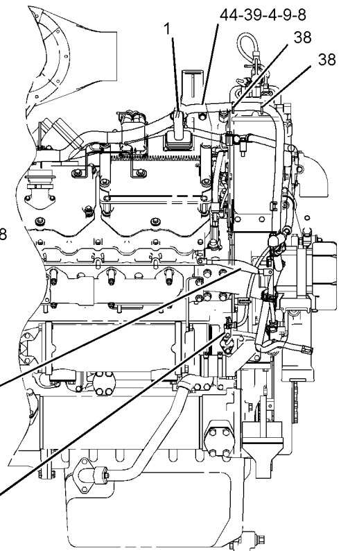
RIGHT SIDE VIEW OF ENGINE
