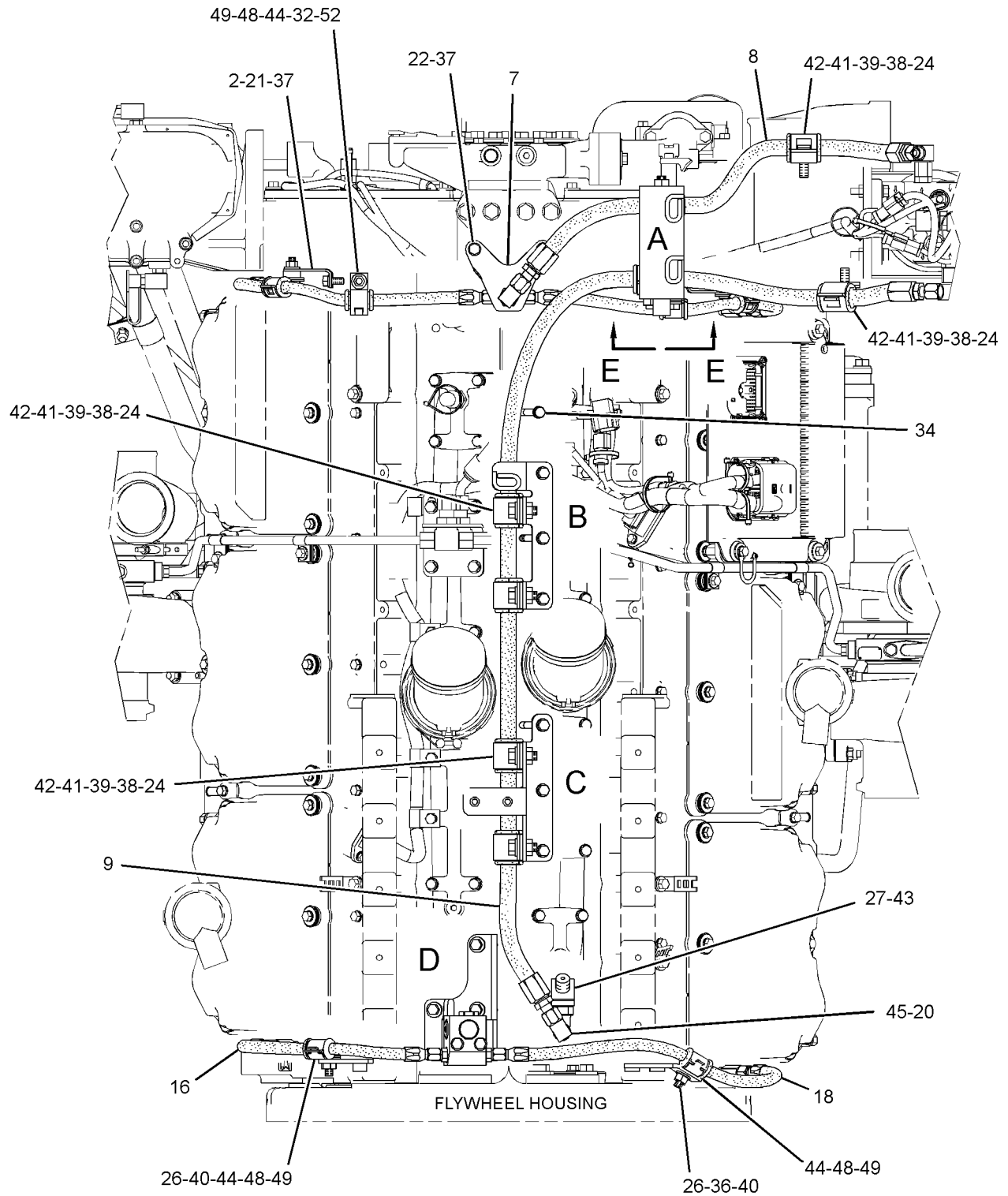
TOP VIEW OF ENGINE
