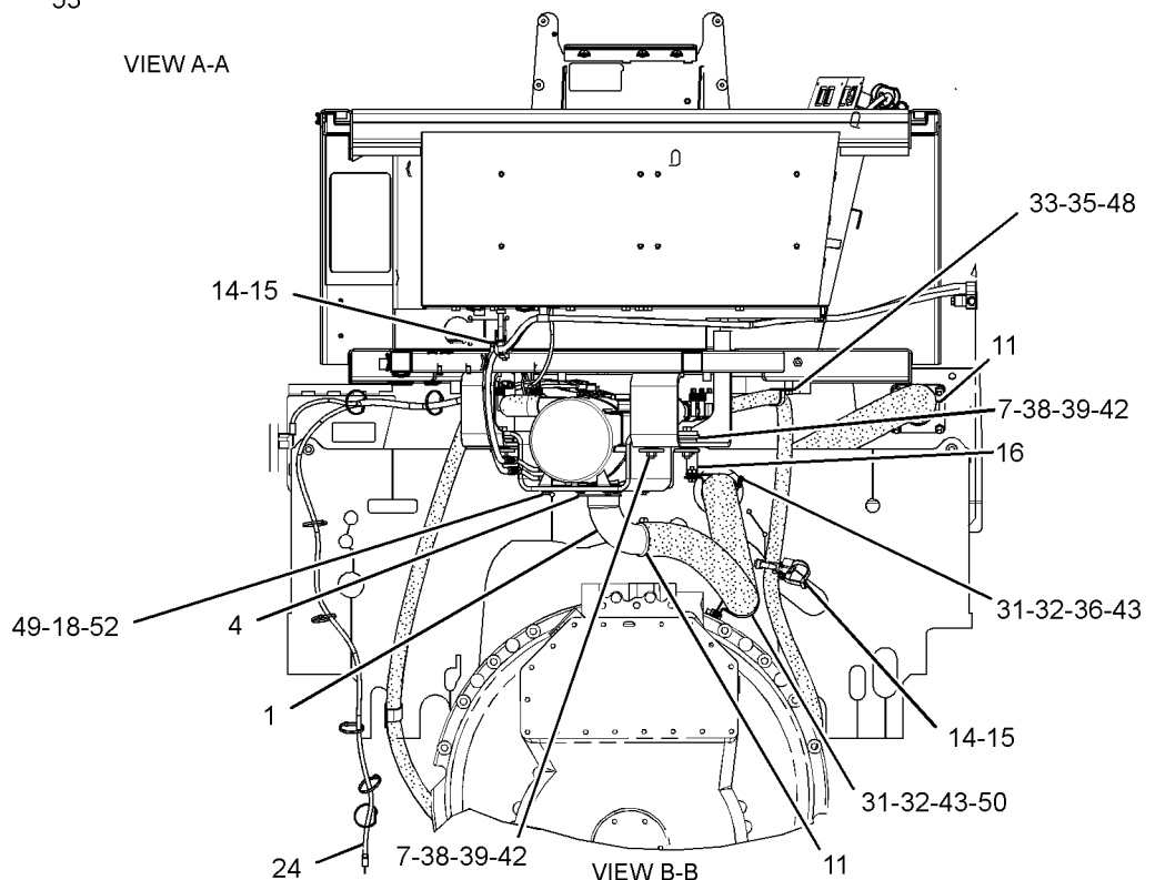
VIEW B-B
