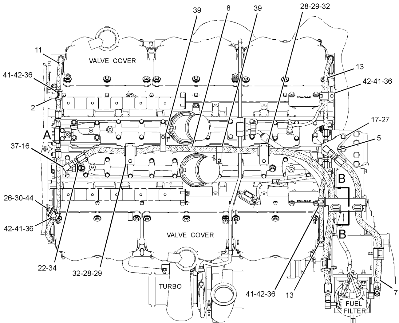
TOP VIEW OF ENGINE
