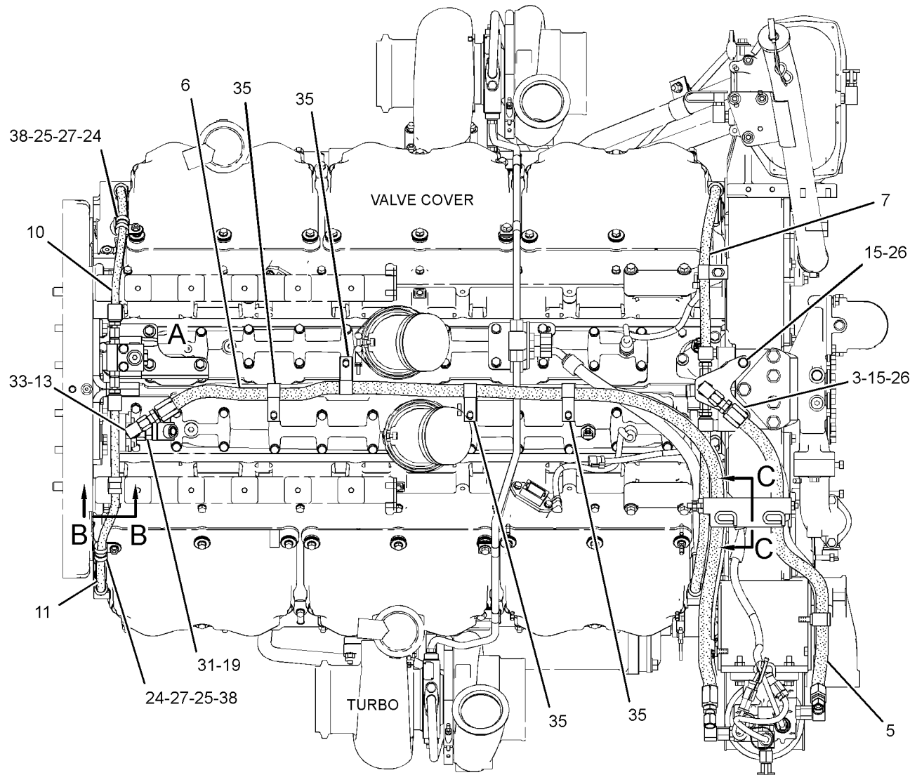
TOP VIEW OF ENGINE
