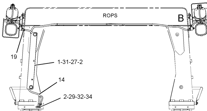
REAR VIEW
