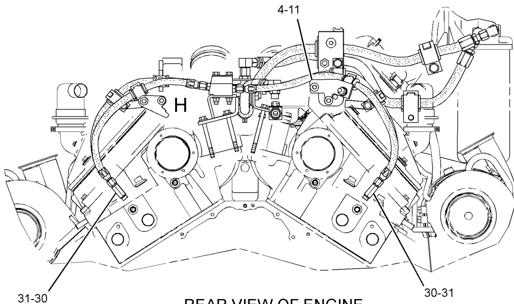
REAR VIEW OF ENGINE
