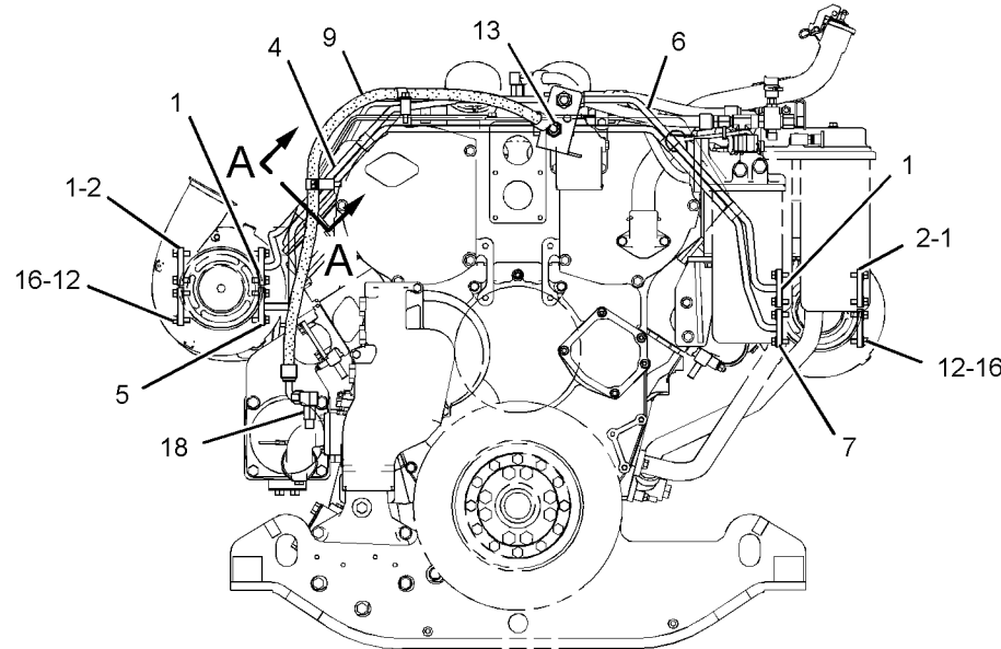
FRONT VIEW <END>
