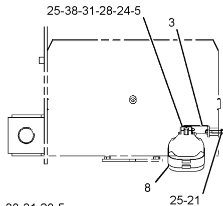
TOP VIEW (REAR FENDER LIGHTS)
