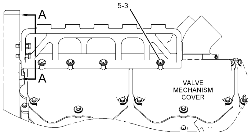
RIGHT SIDE VIEW OF ENGINE
