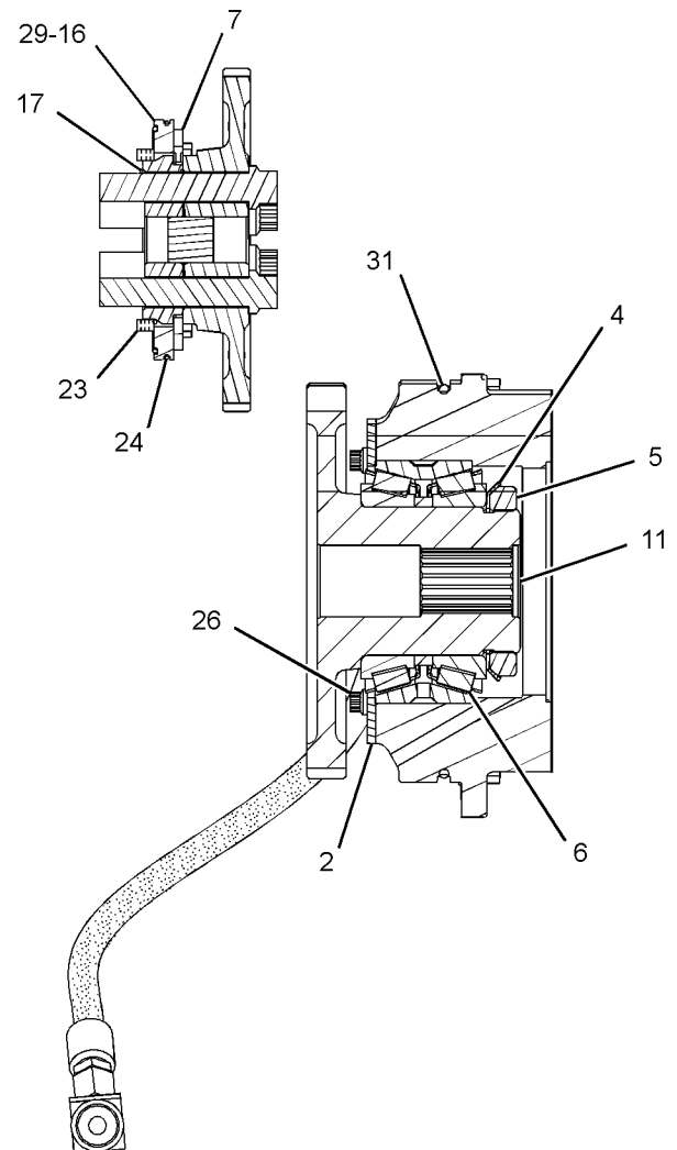
SECTION B-B
