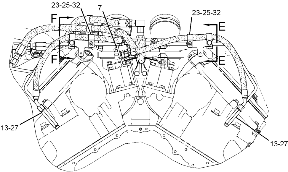
REAR VIEW <END>
