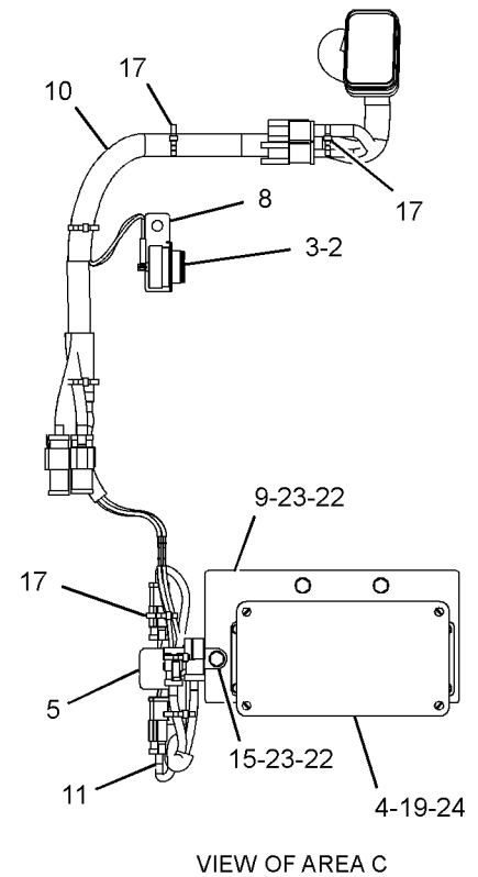
VIEW OF AREA C
