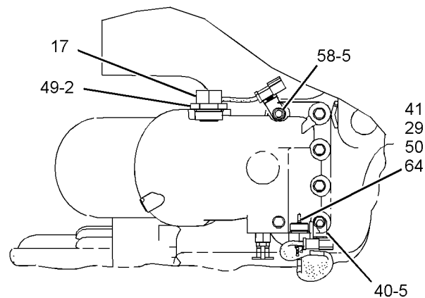
VIEW G-G
