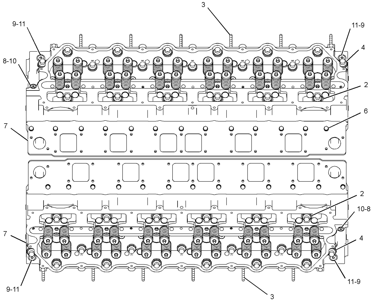
TOP VIEW
