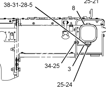
FRONT VIEW (FRONT FENDER LIGHTS)
