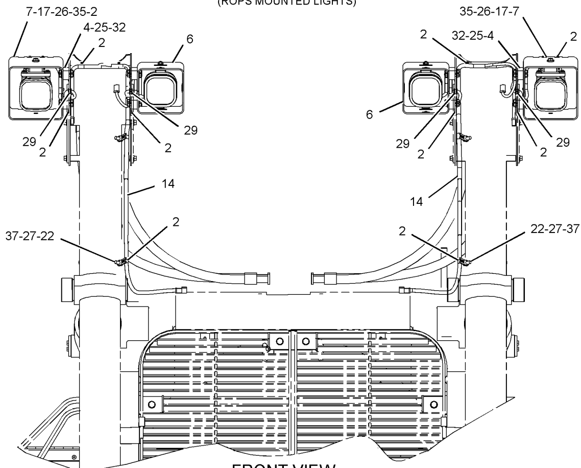
FRONT VIEW (CYLINDER MOUNTED LIGHTS)
