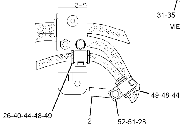
VIEW E-E
