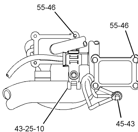
VIEW E-E
