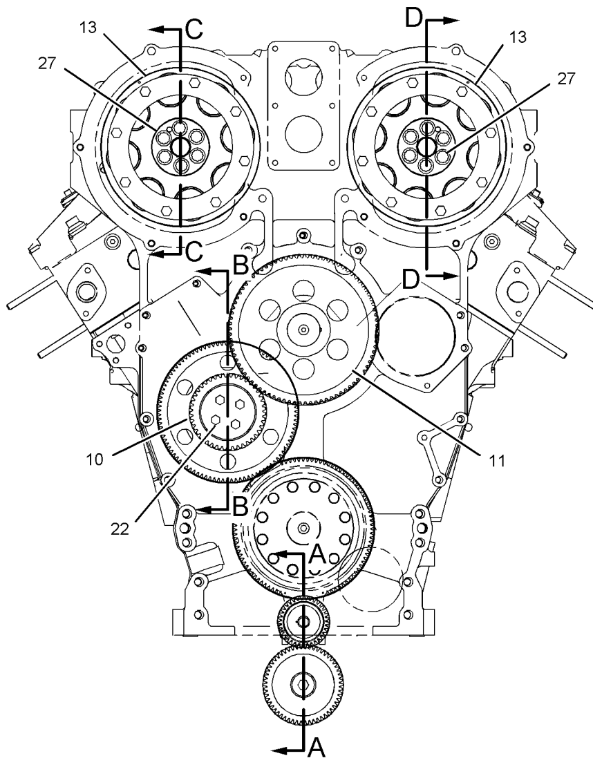
FRONT VIEW
