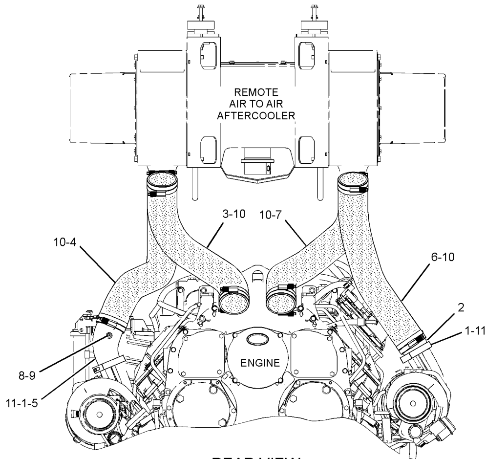
REAR VIEW
