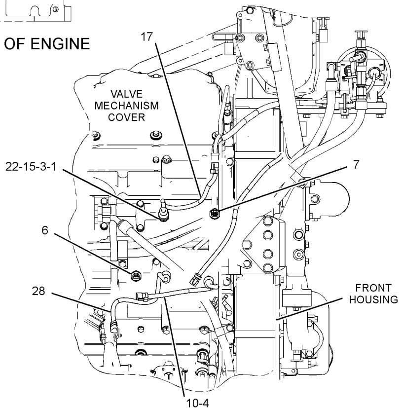
TOP VIEW OF ENGINE
