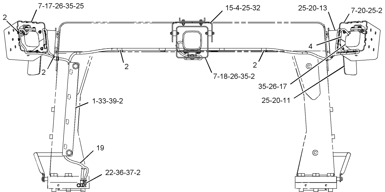
REAR VIEW (ROPS MOUNTED LIGHTS)
