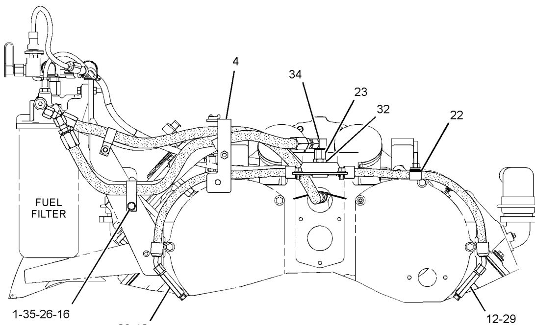
FRONT VIEW OF ENGINE
