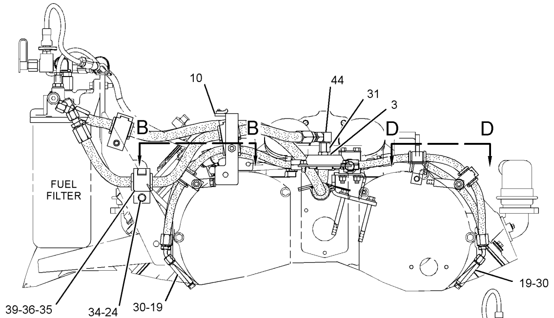
FRONT VIEW OF ENGINE
