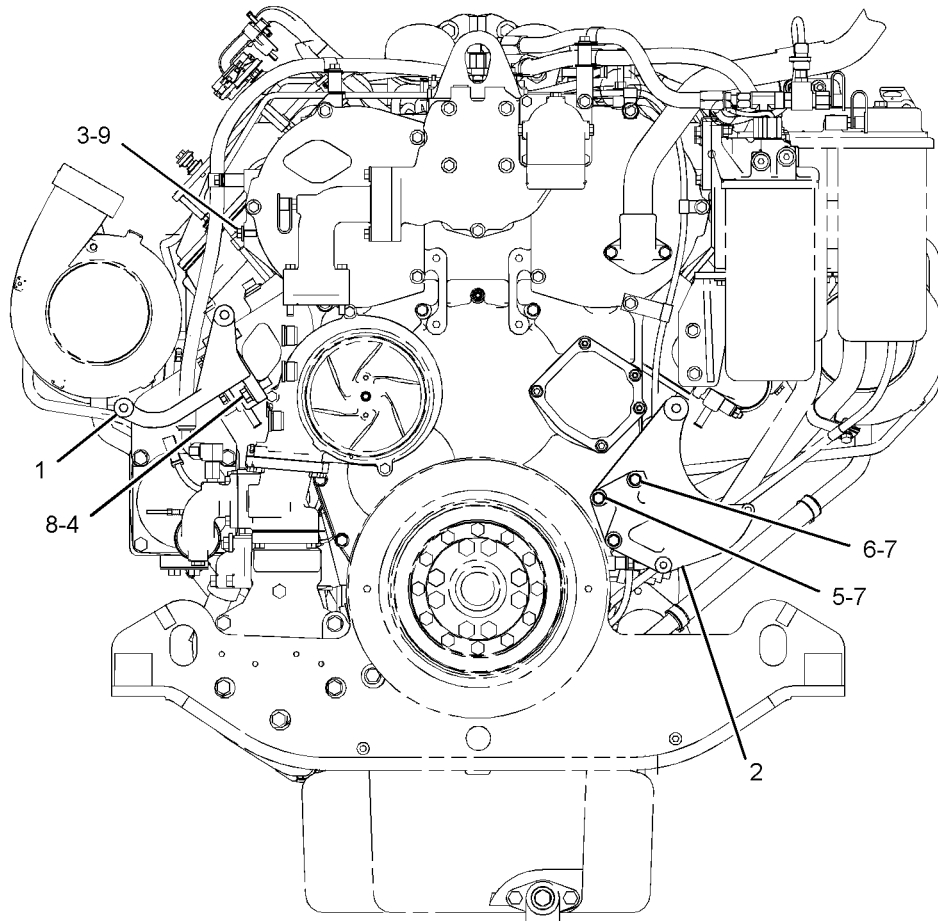
FRONT VIEW
