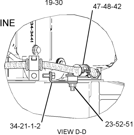
VIEW D-D
