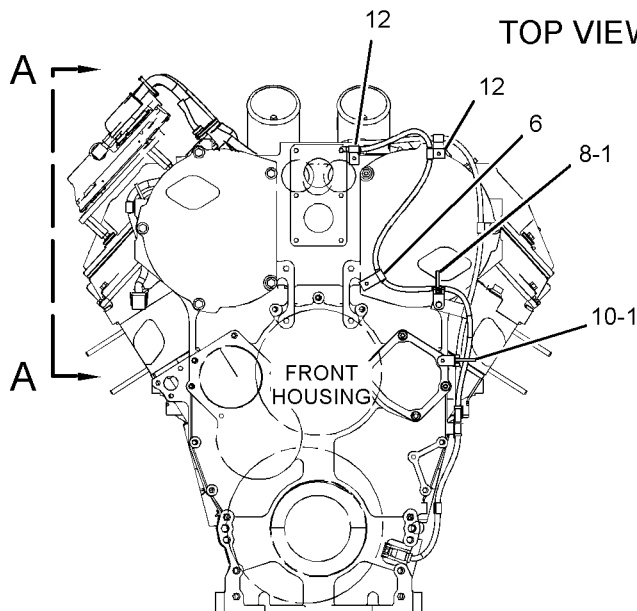
FRONT VIEW OF ENGINE
