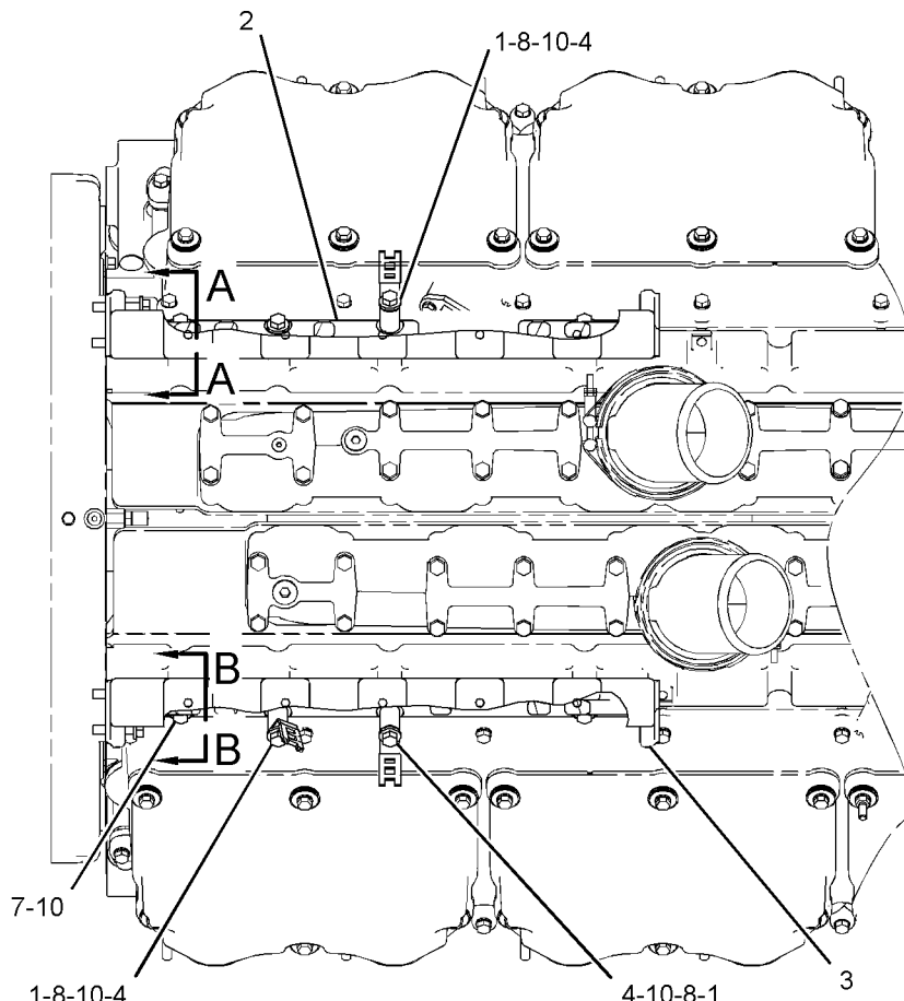
TOP VIEW OF ENGINE
