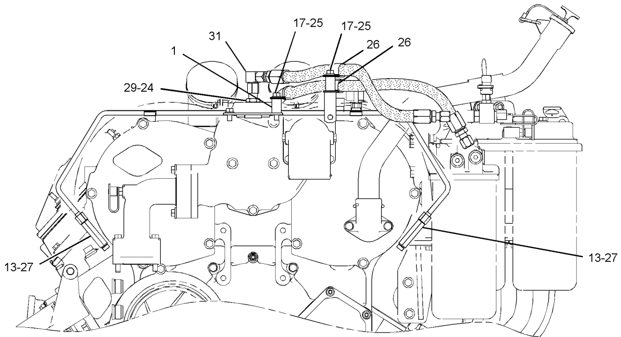
FRONT VIEW
