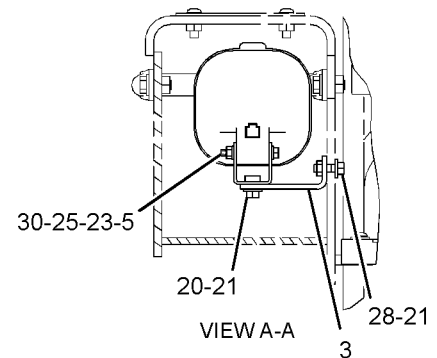
(VIEW OF RH CONSOLE)
