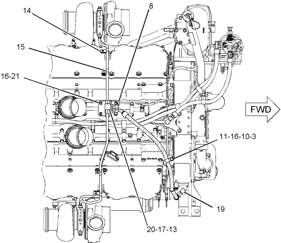
TOP VIEW
