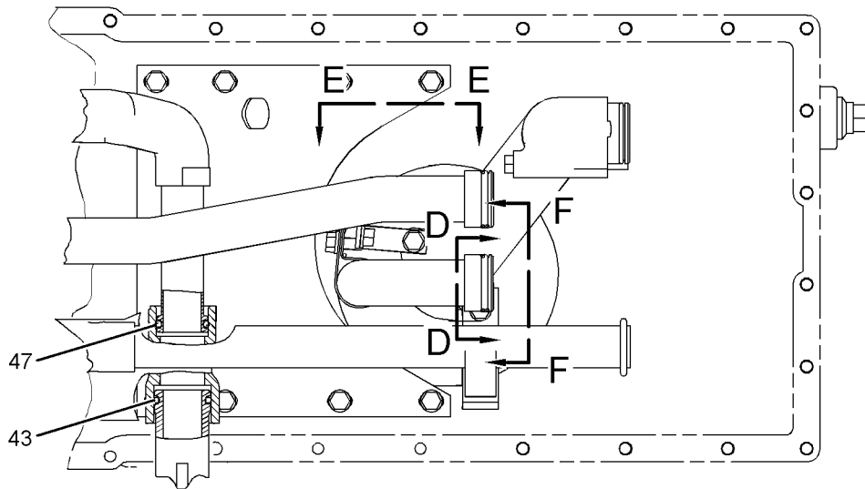
VIEW OF AREA B
