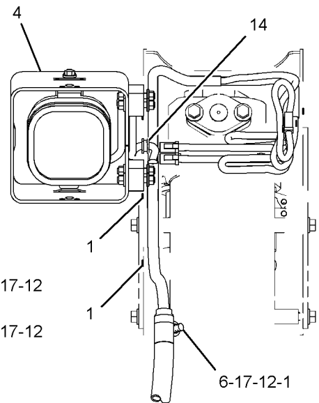
VIEW OF AREA B
