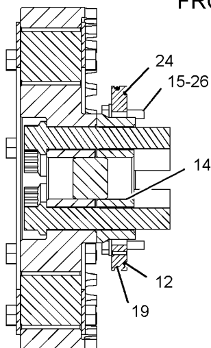
SECTION C-C
