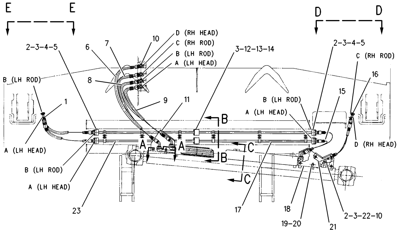
REAR VIEW
