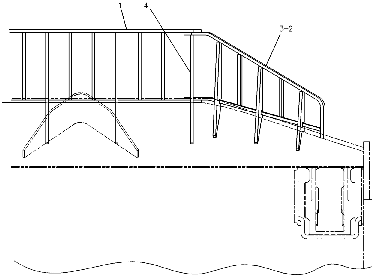
REAR VIEW
