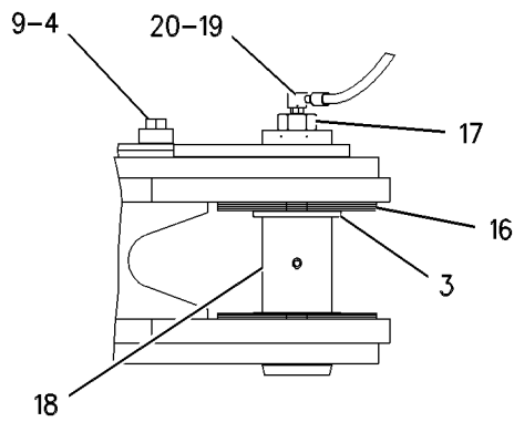
VIEW D-D
