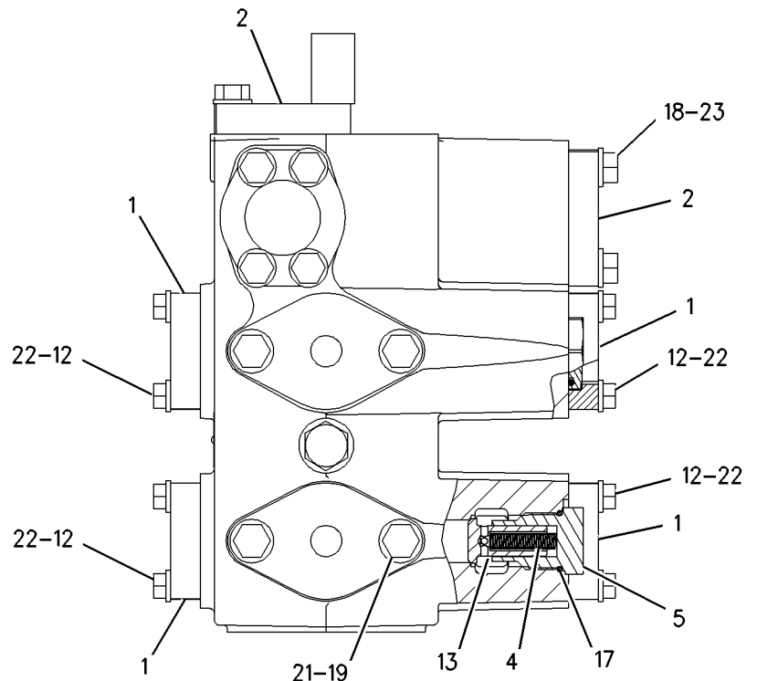
VIEW OF AREA A ALTERNATE INSTALLATION ROTATED 180 DEGREES
