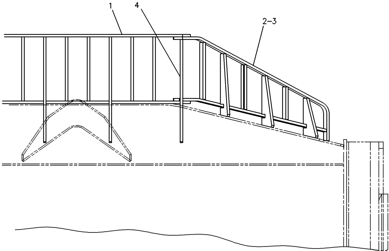
REAR VIEW
