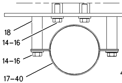
VIEW C-C
