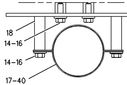
VIEW C-C
