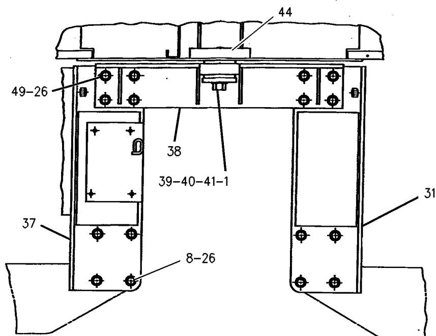
VIEW B-B
