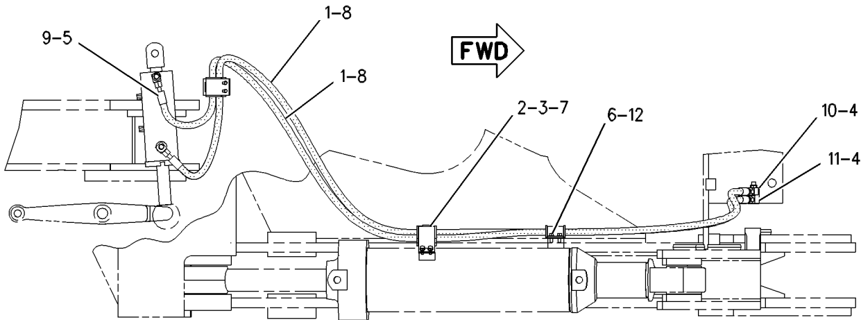
TOP VIEW
