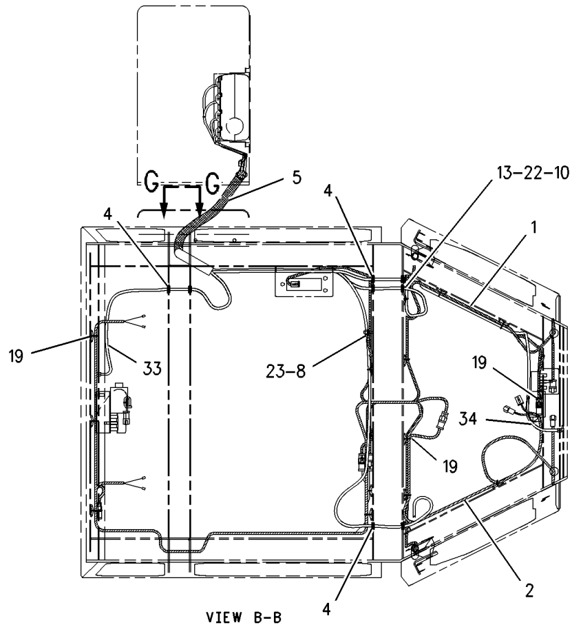
VIEW B-B
