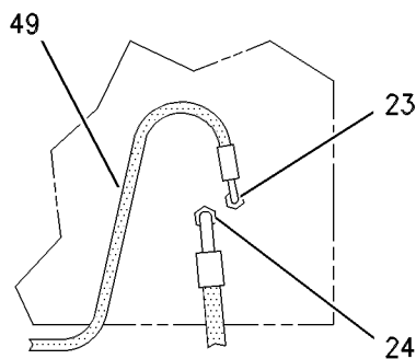
VIEW D-D
