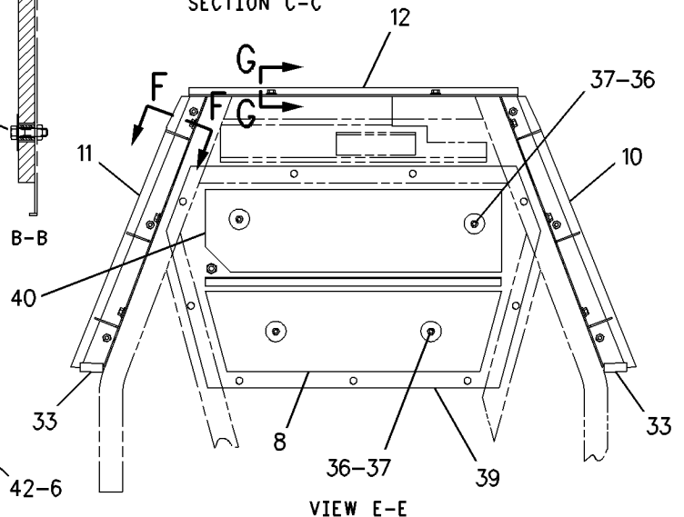
VIEW E-E
