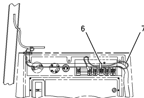
VIEW C-C
