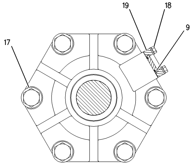
SECTION B-B
