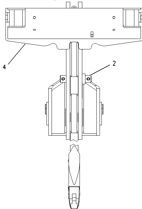
REAR VIEW
