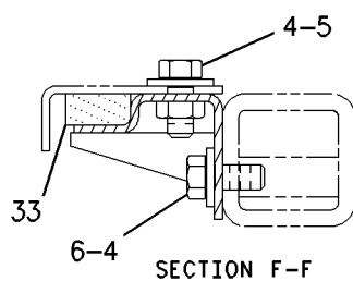
SECTION F-F
