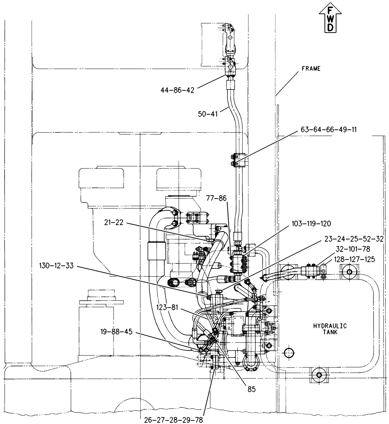
TOP VIEW
