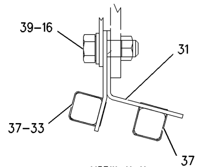
VIEW K-K
