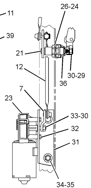
VIEW D-D
