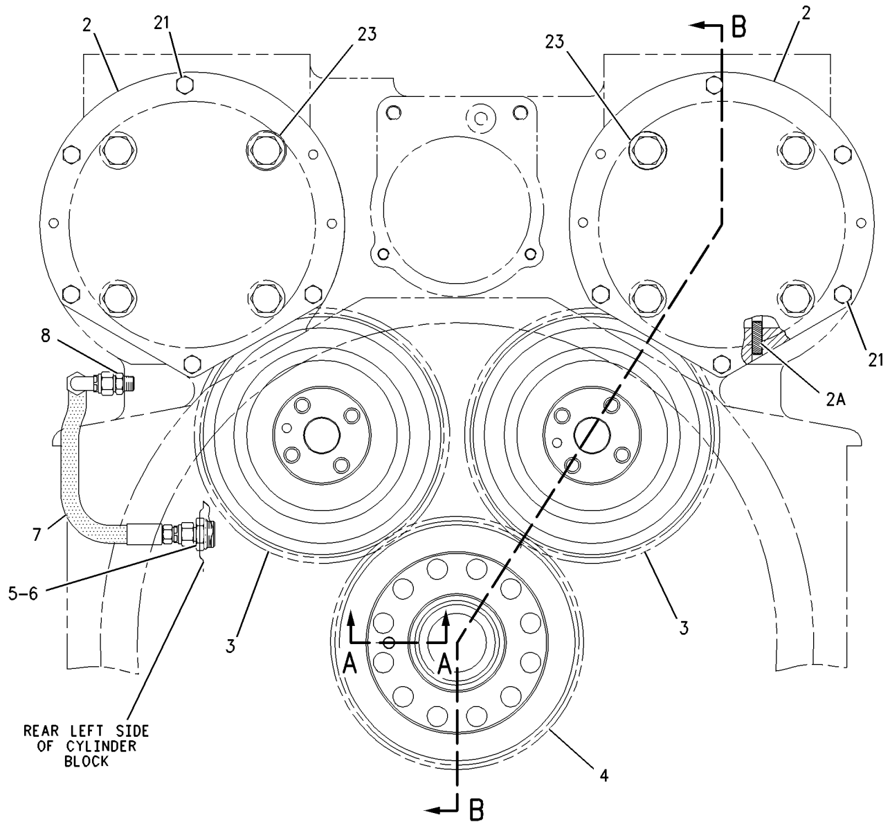
REAR VIEW
