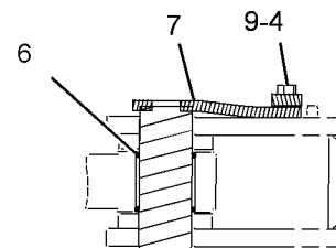
VIEW E-E
