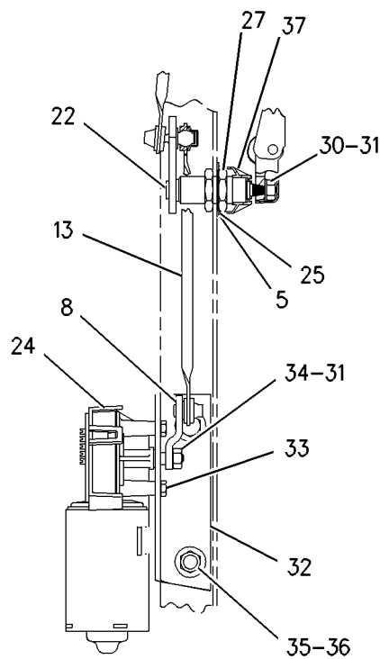
VIEW E-E
