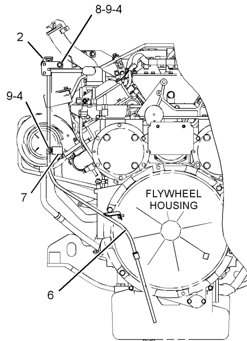
REAR VIEW
