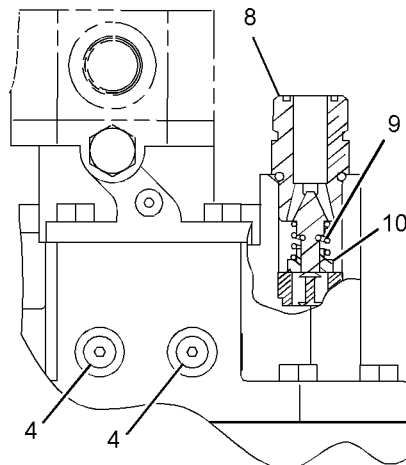
VIEW E-E
