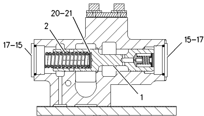
SECTION C-C (ROTATED 90 DEGREES CCW)
