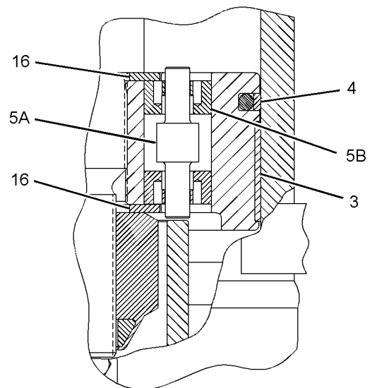
VIEW OF AREA B
