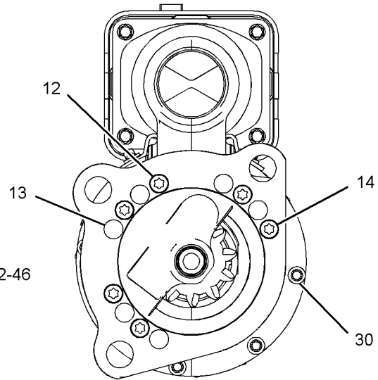
REAR VIEW OF ENGINE
