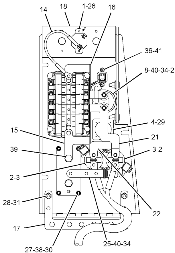
VIEW B-B (HARNESS REMOVED)
