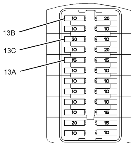
FUSE BOX
