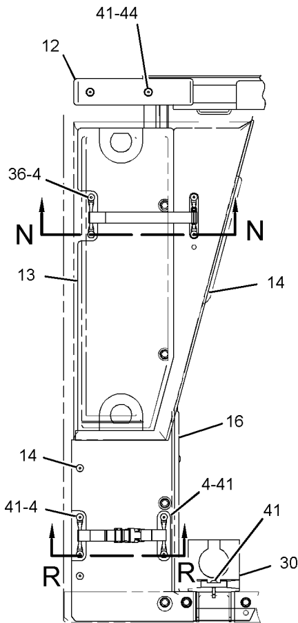
VIEW M-M
