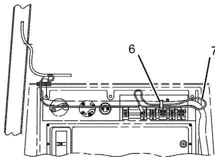
VIEW C-C
