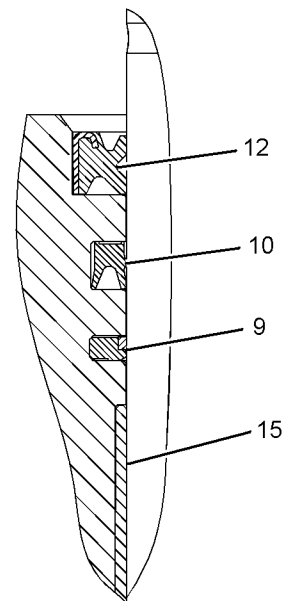
VIEW OF AREA B
