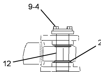
VIEW F-F
