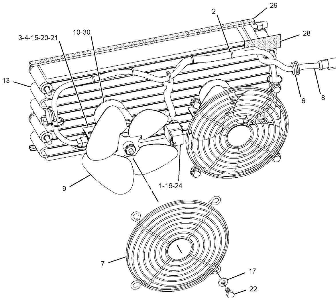
VIEW OF AREA A (COVER AND MOUNTING HARDWARE REMOVED)
