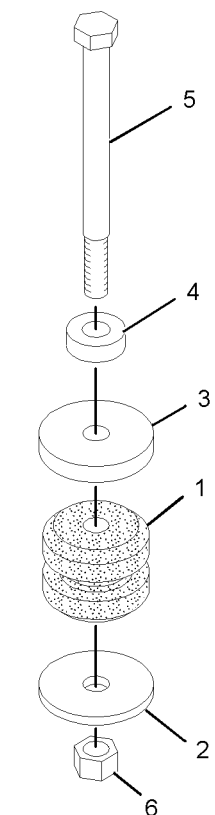
VIEW OF AREA A (EXPLODED)
