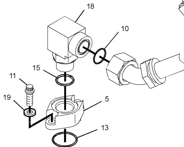
VIEW OF AREA B EXPLODED
