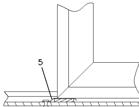
SECTION VIEW OF AREA B
