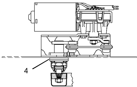
VIEW E-E
