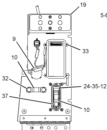
SECTION C-C
