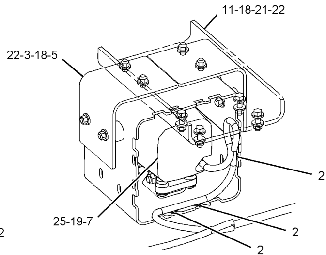
VIEW OF AREA D
