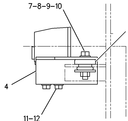
VIEW B-B
