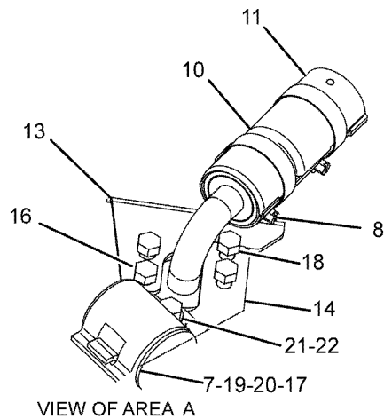
VIEW OF AREA A
