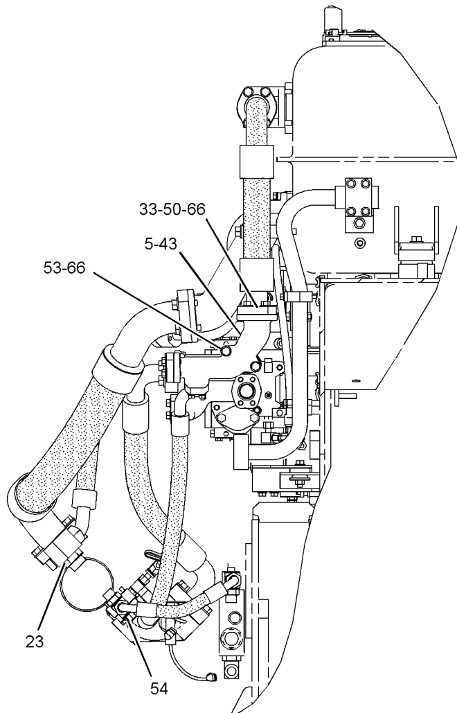
REAR VIEW
