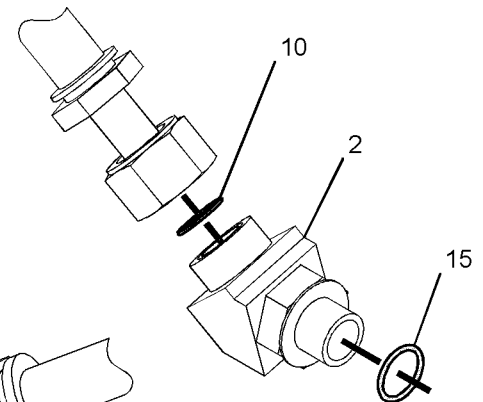
VIEW OF AREA A EXPLODED
