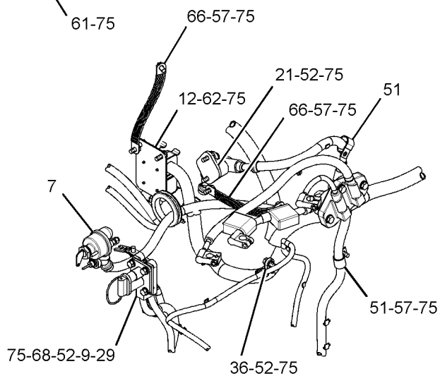
VIEW OF AREA E
