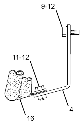
VIEW OF AREA B
