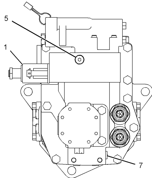
VIEW C-C
