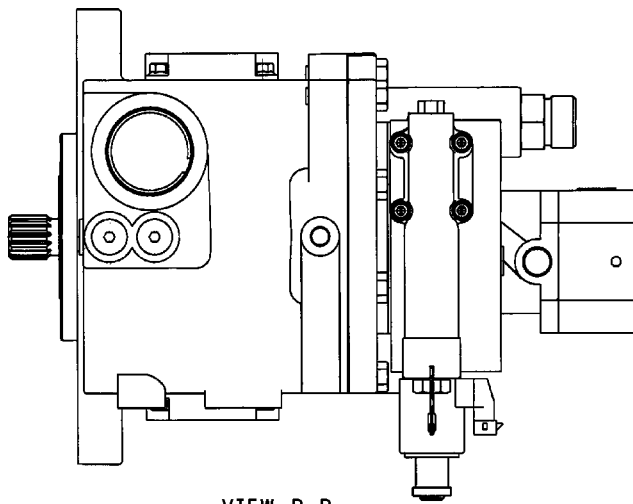
VIEW B-B
