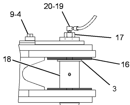
VIEW D-D
