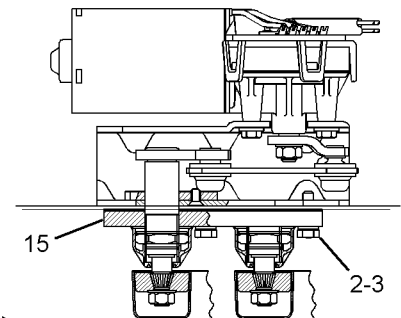
VIEW C-C
