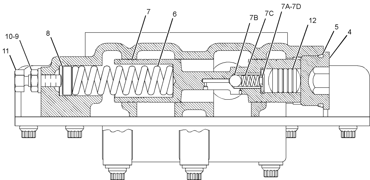
SECTION B-B
