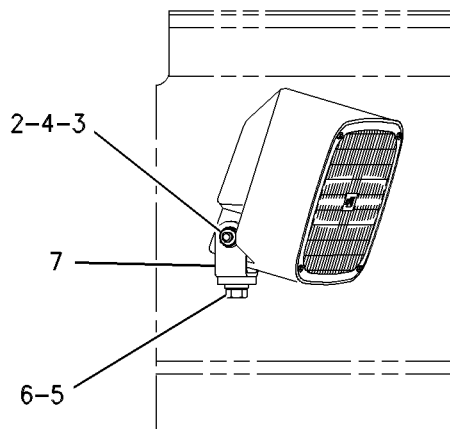
VIEW B-B
