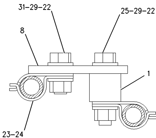
SECTION C-C
