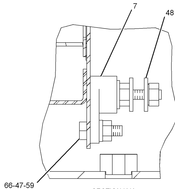
SECTION K-K
