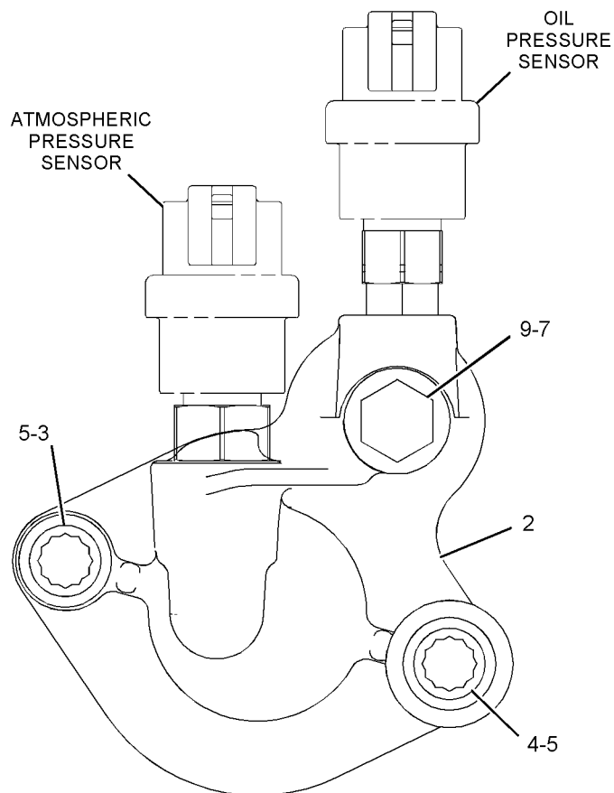
LEFT SIDE VIEW OF ENGINE
