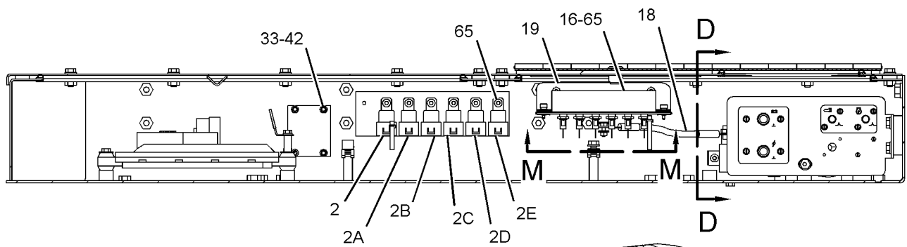
SECTION E-E
