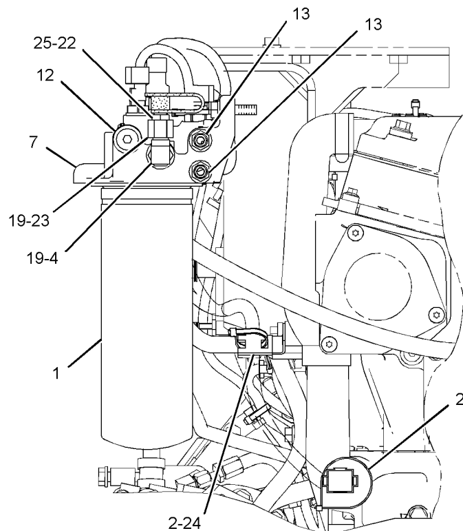
REAR VIEW OF ENGINE
