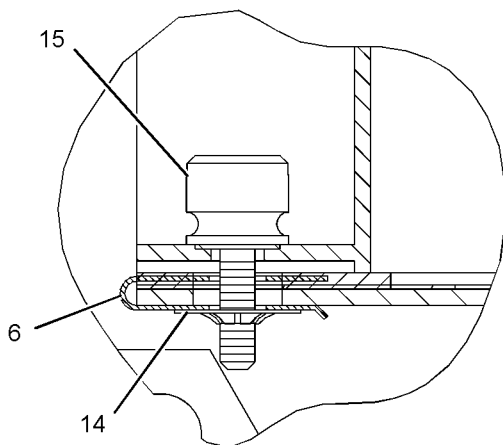
SECTION N-N
