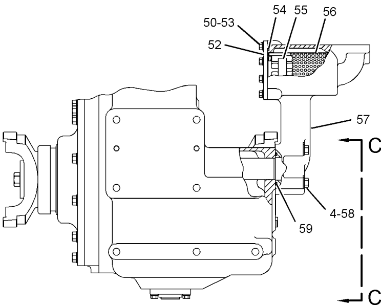
VIEW B-B
