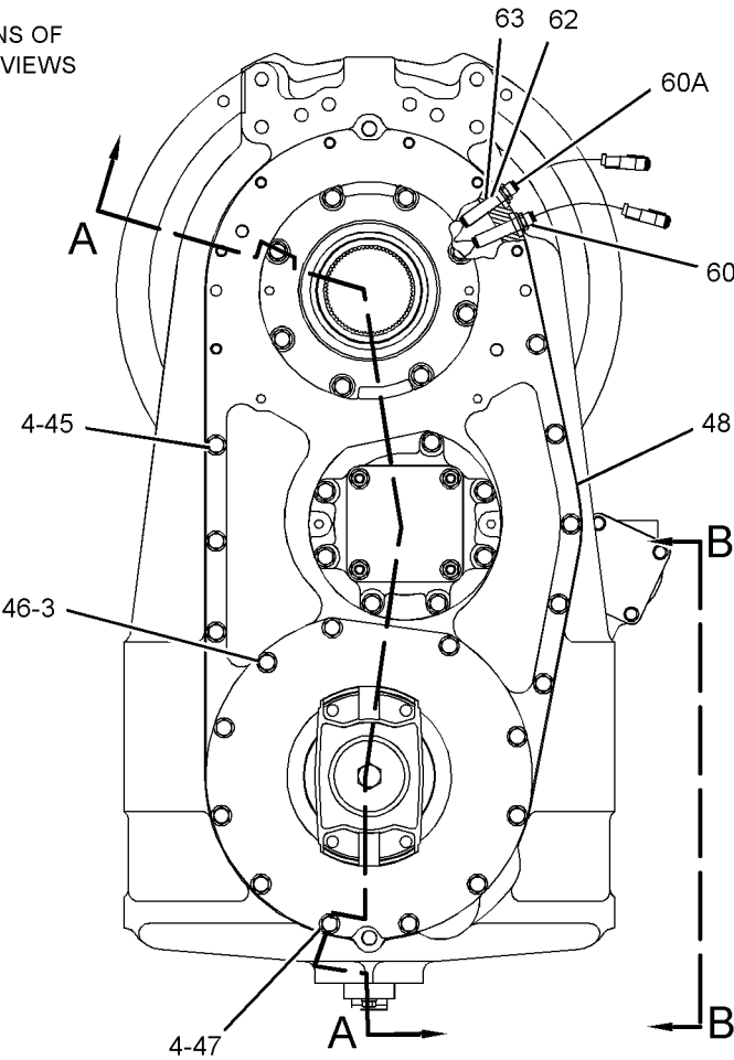
FRONT VIEW
