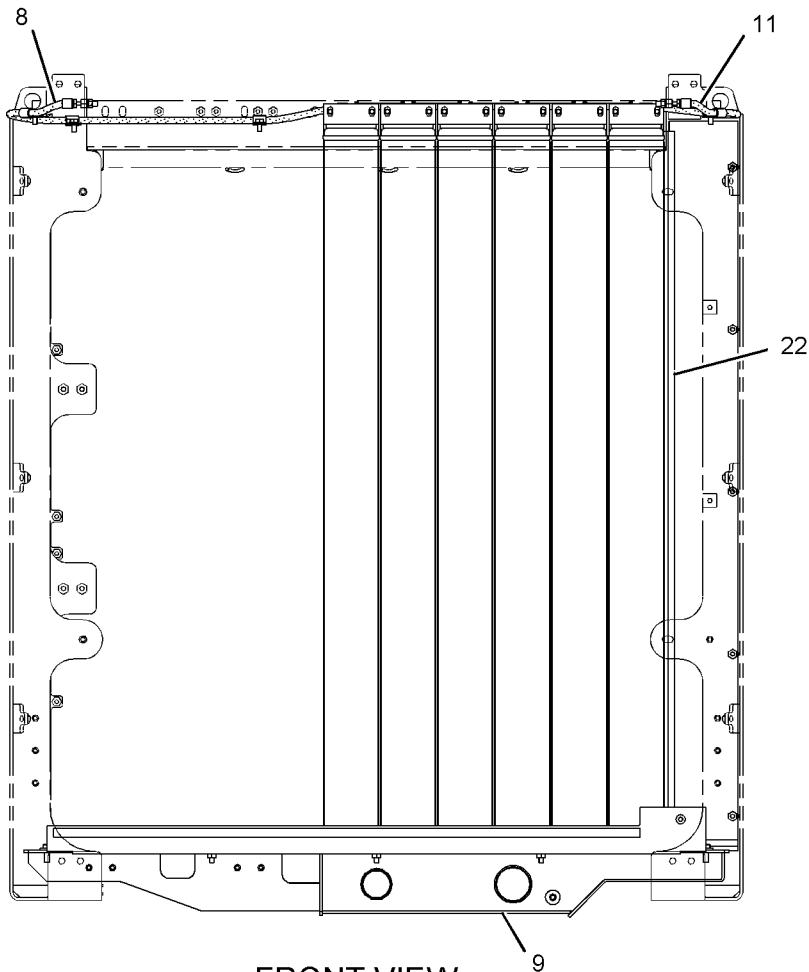
FRONT VIEW
