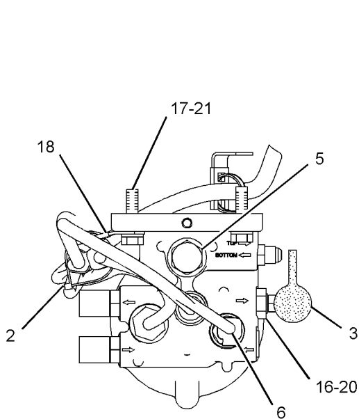
TOP VIEW OF ENGINE
