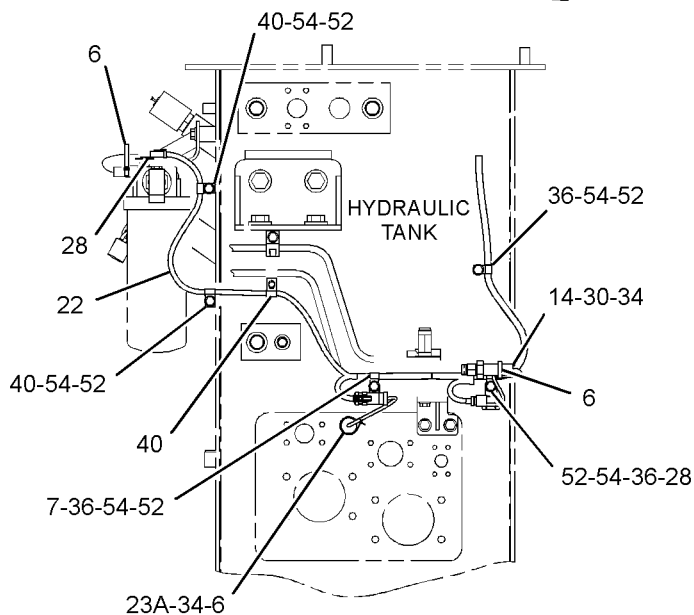
SECTION G
