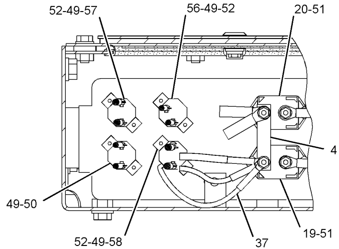
SECTION U-U
