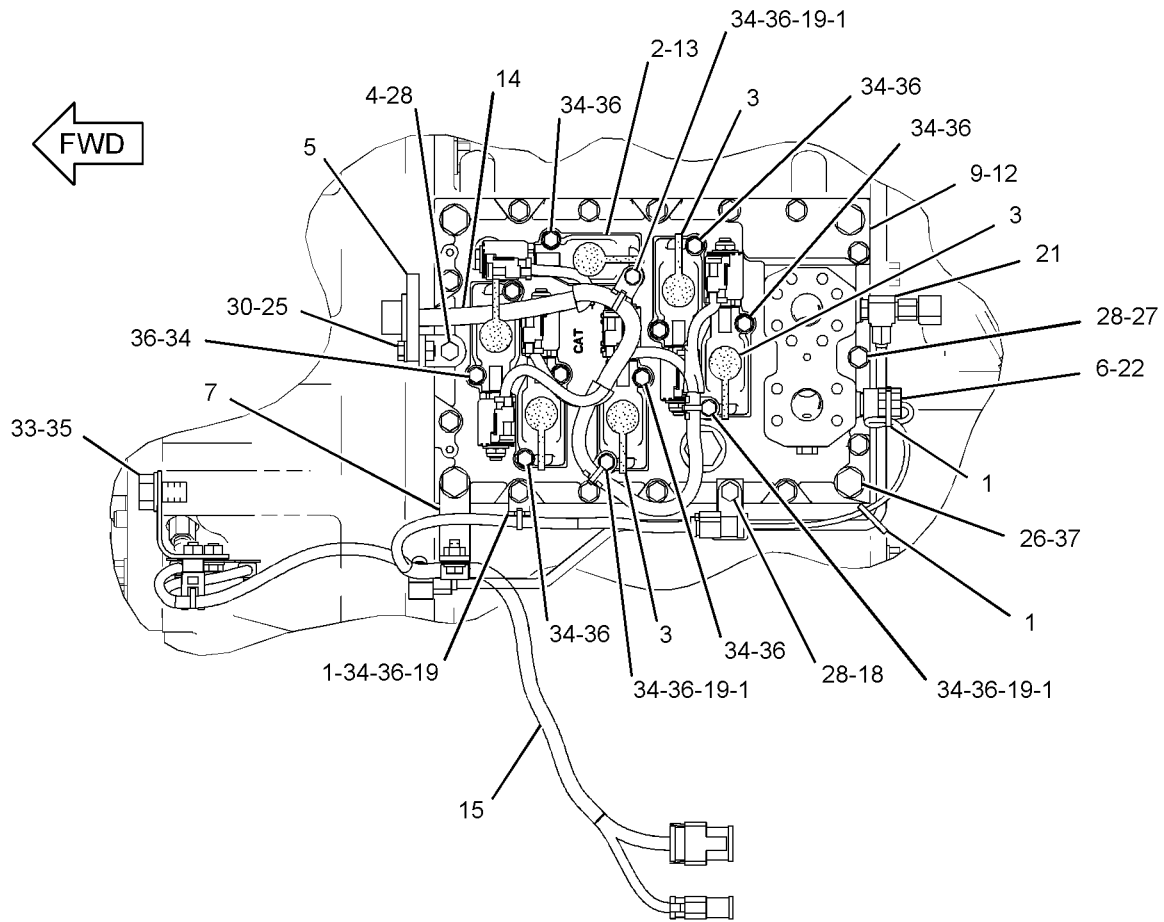
TOP VIEW
