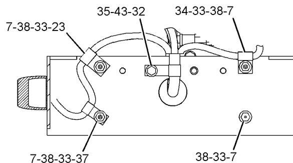
SECTION L-L
