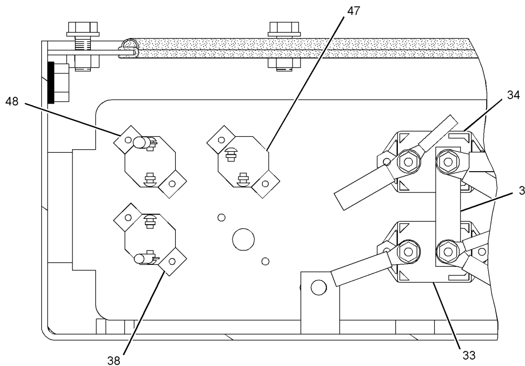
SECTION J-J
