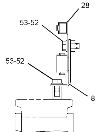
VIEW W-W
