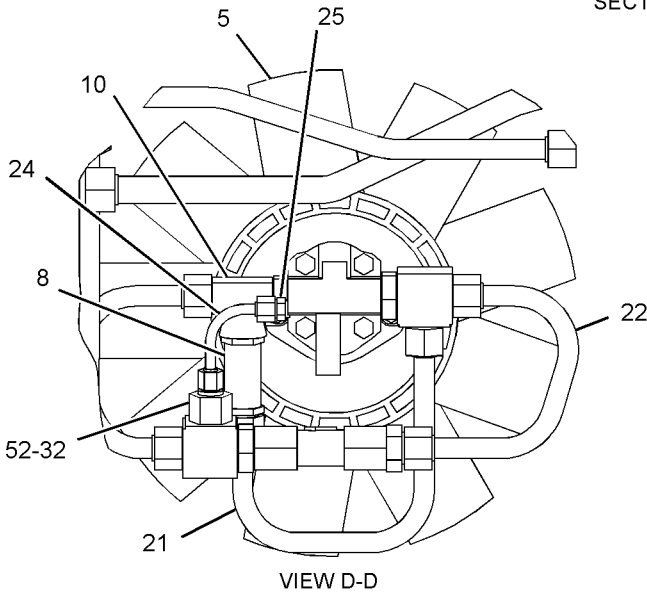
VIEW D-D
