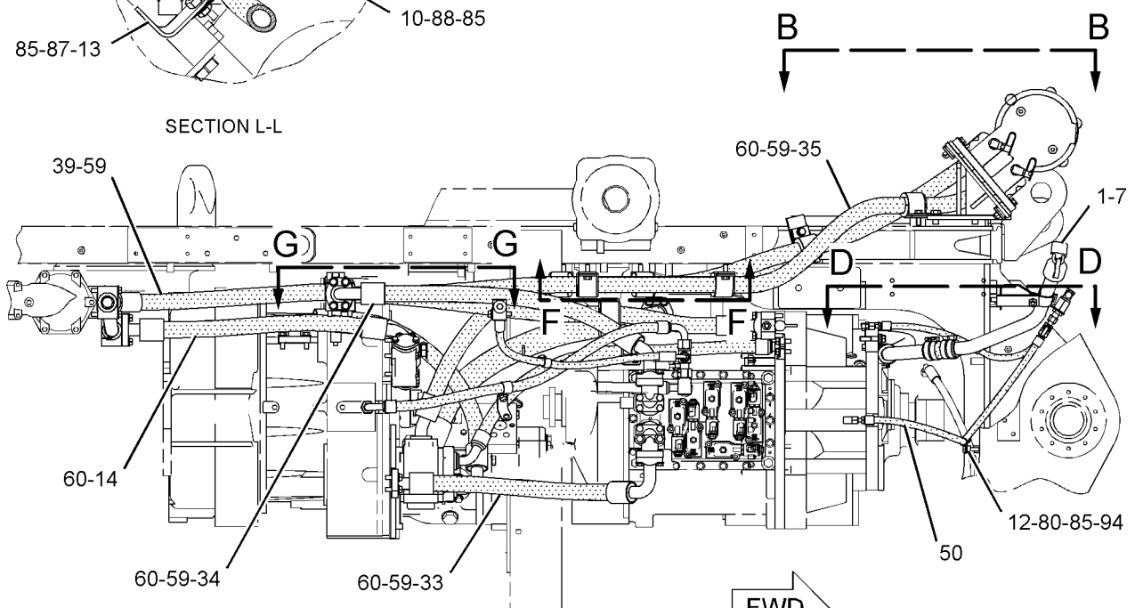
TOP VIEW
