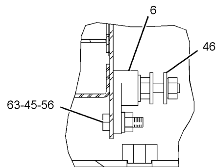
SECTION K-K
