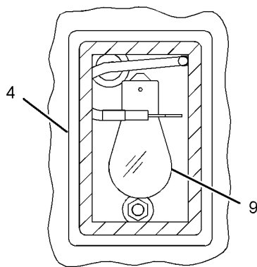
SECTION E-E
