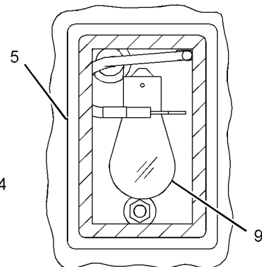
SECTION F-F
