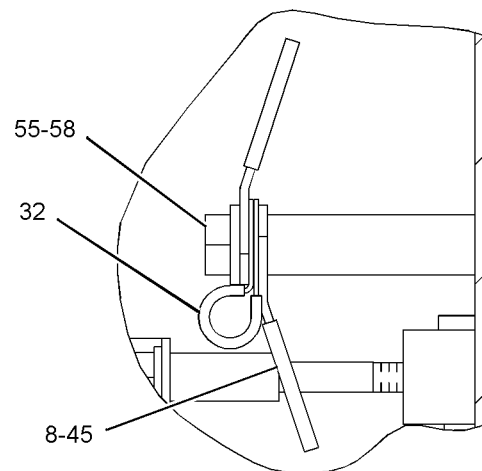
SECTION H-H
