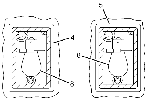
SECTION E-E
