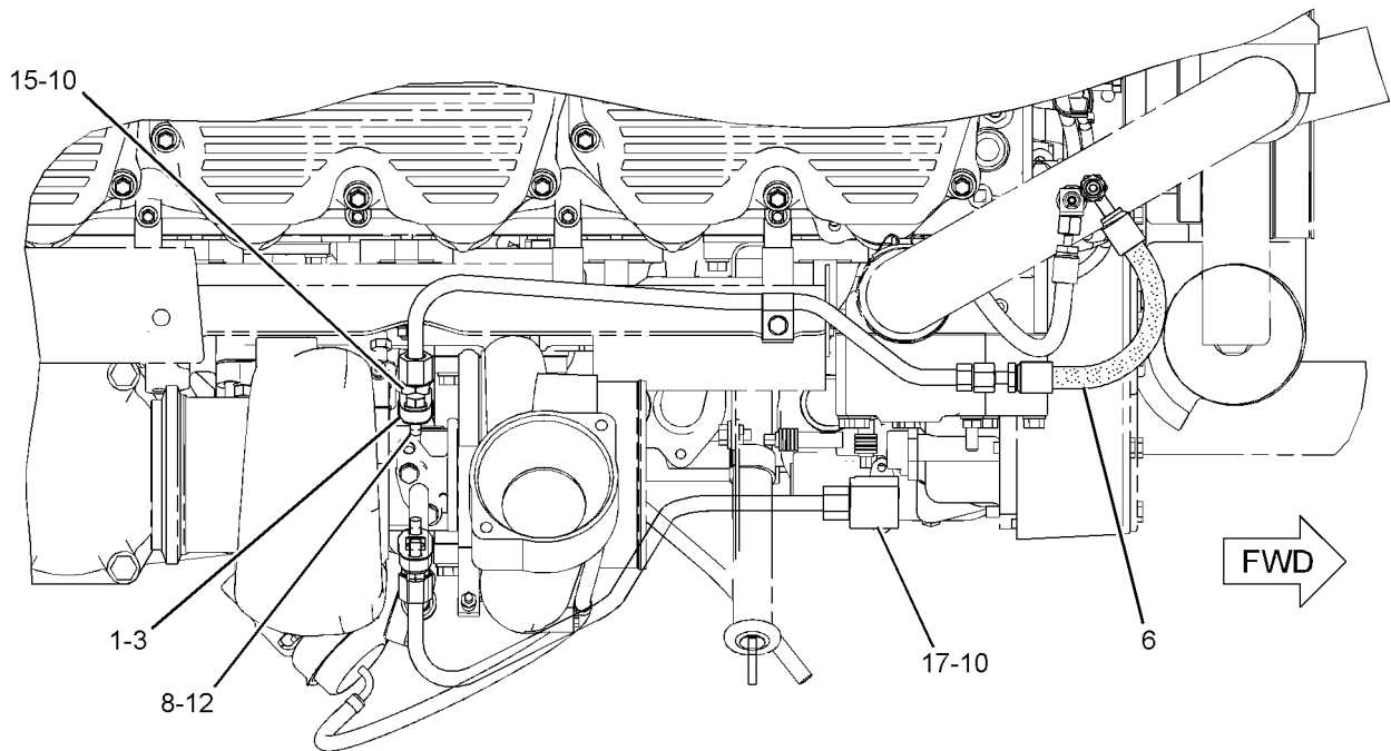
TOP VIEW
