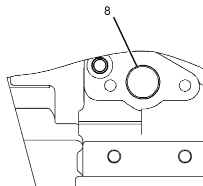
VIEW E-E
