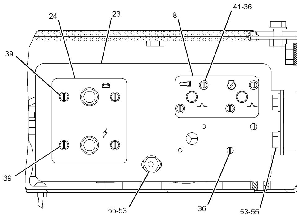
SECTION L-L
