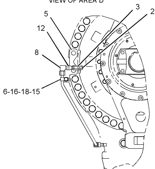
VIEW E-E
