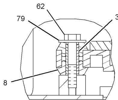
SECTION P-P
