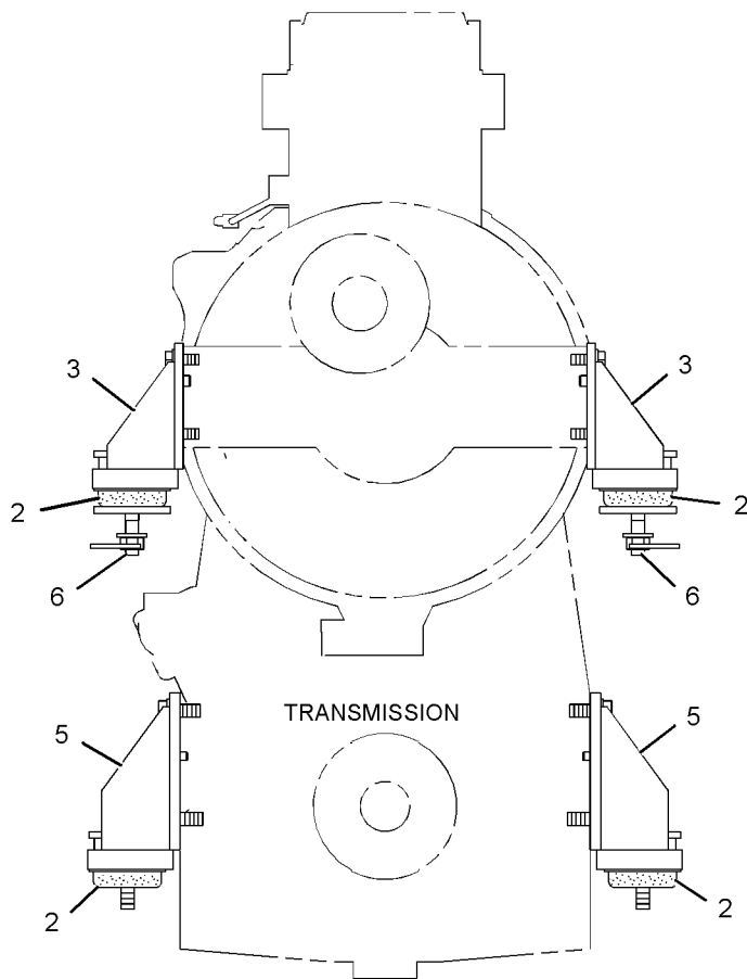
REAR VIEW
