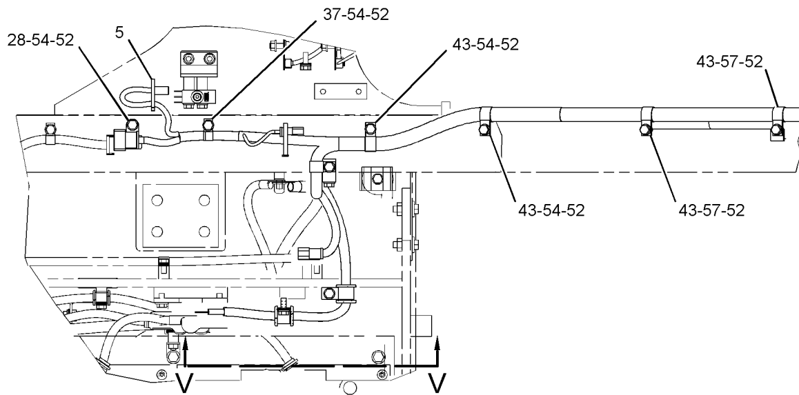
SECTION C-C
