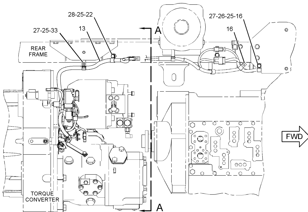
TOP VIEW
