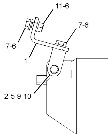
VIEW D-D
