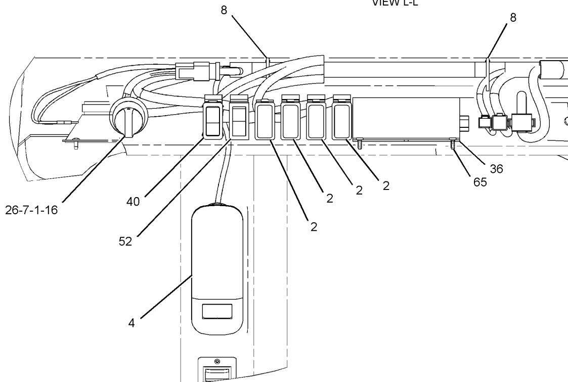
VIEW L-L
