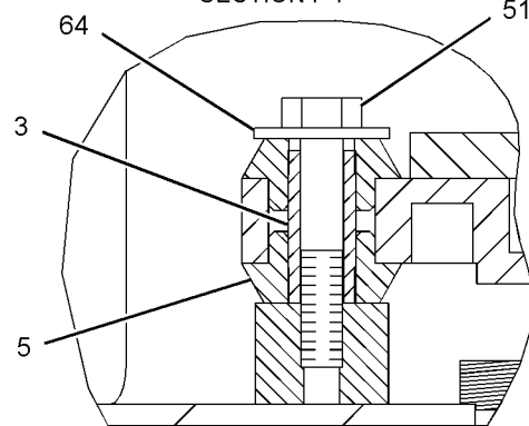
SECTION P-P
