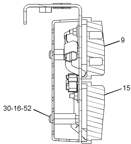
SECTION K-K
