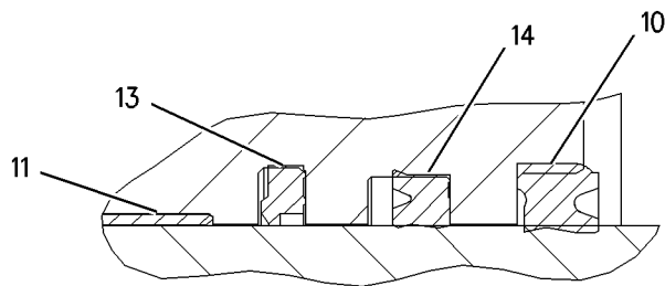
VIEW OF AREA A
