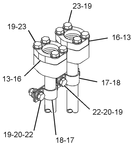
VIEW OF AREA B
