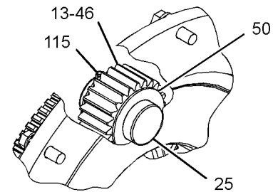
VIEW OF AREA S
