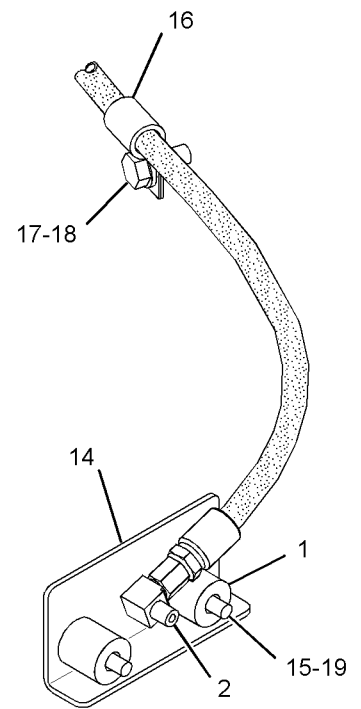
VIEW OF AREA C
