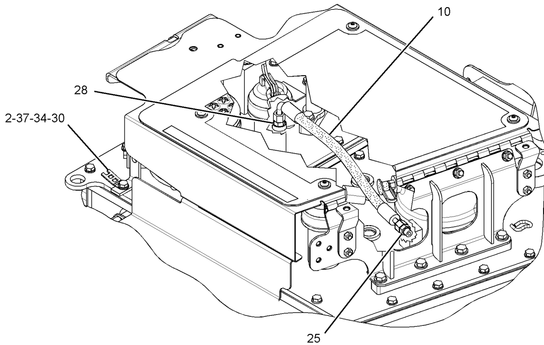
VIEW OF AREA C
