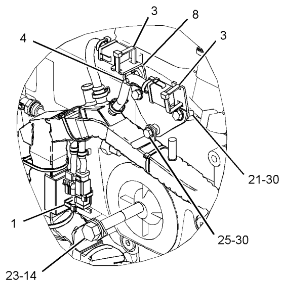
VIEW OF AREA C
