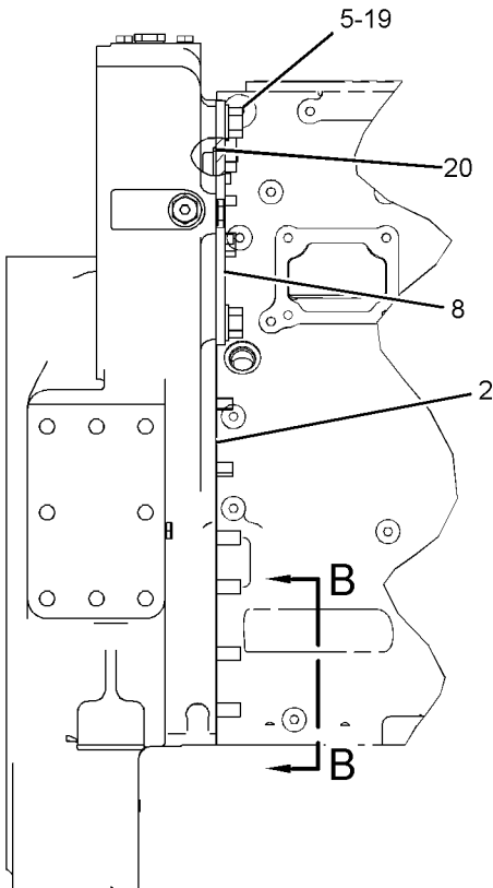
RIGHT SIDE VIEW OF ENGINE
