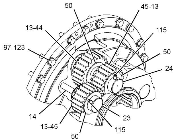
VIEW OF AREA T
