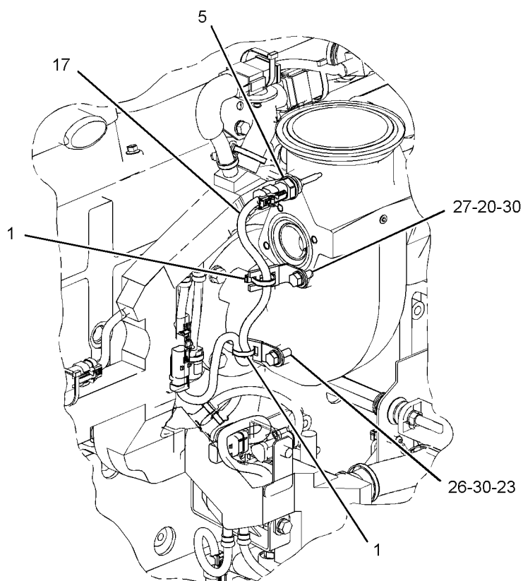
VIEW OF AREA D
