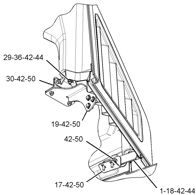
VIEW OF AREA B (PARTS REMOVED FOR CLARITY)
