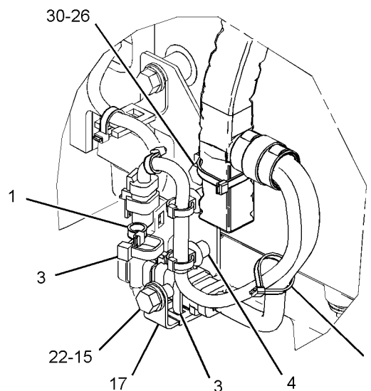
VIEW OF AREA E
