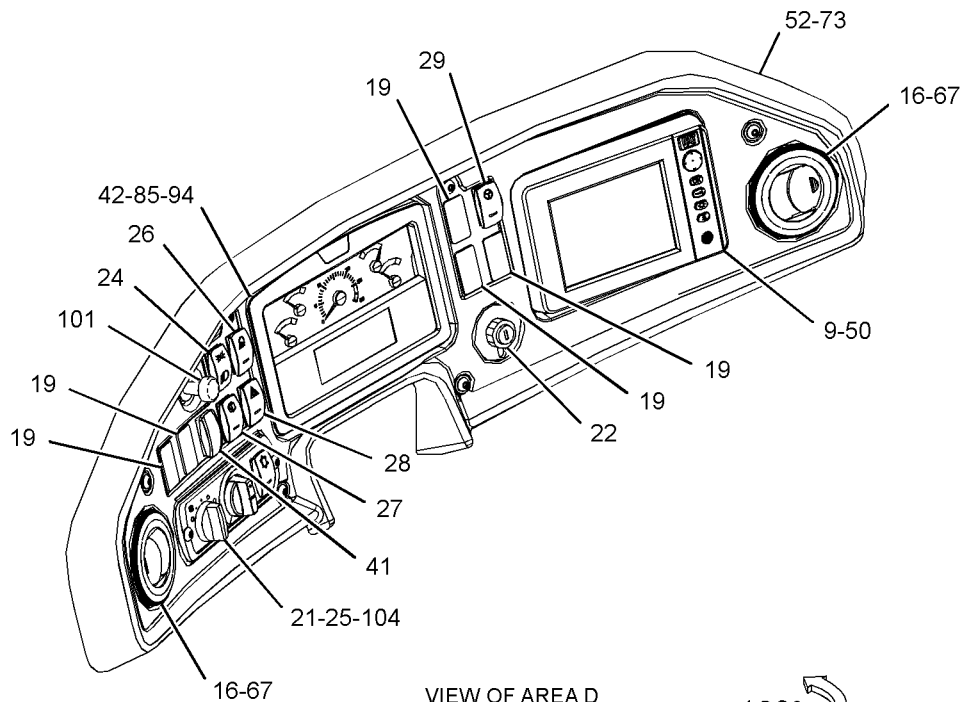
VIEW OF AREA D (PARTS REMOVED FOR CLARITY)
