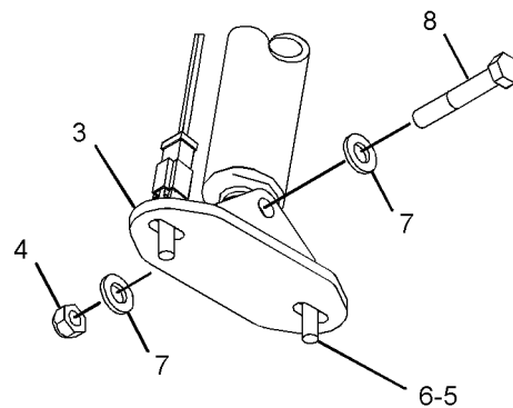
VIEW OF AREA B
