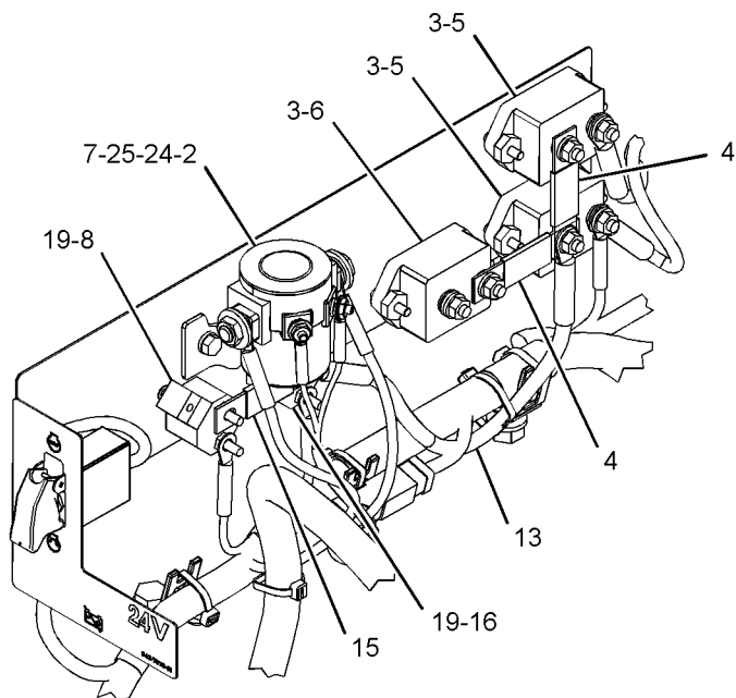
VIEW OF AREA A
