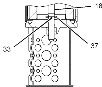
VIEW OF AREA C
