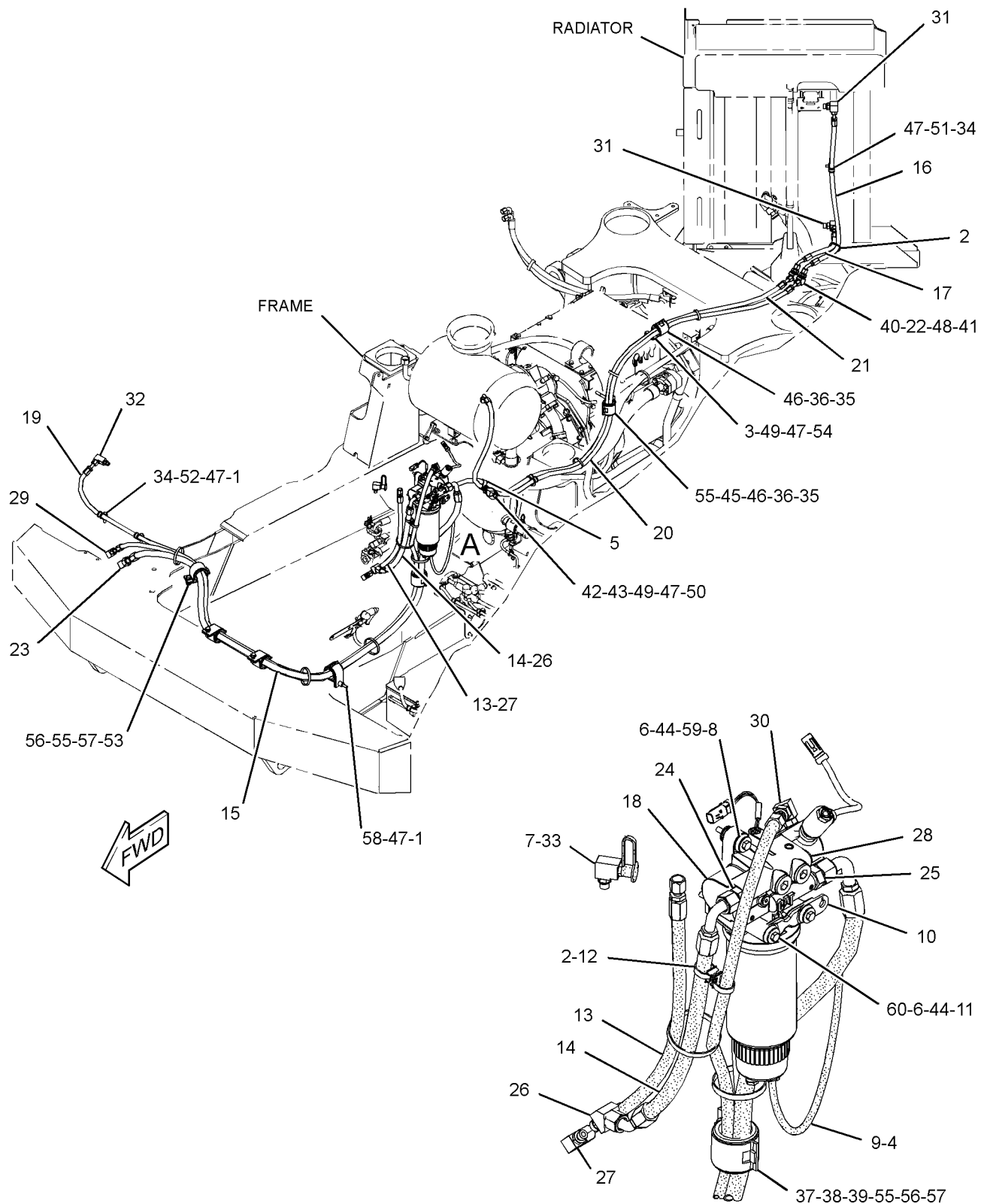
VIEW OF AREA A
